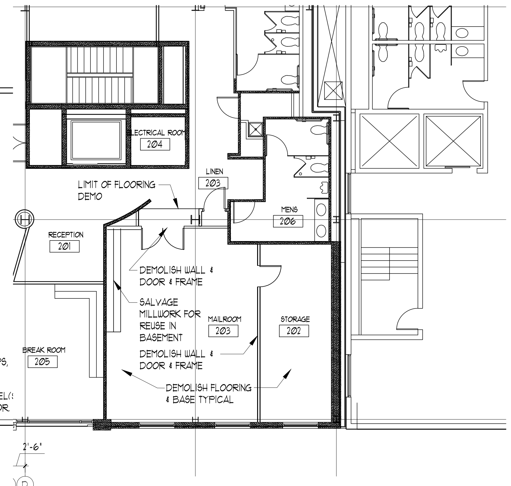
2ND FLOOR DEMO SCALE: 1/8" = 1'-0"
