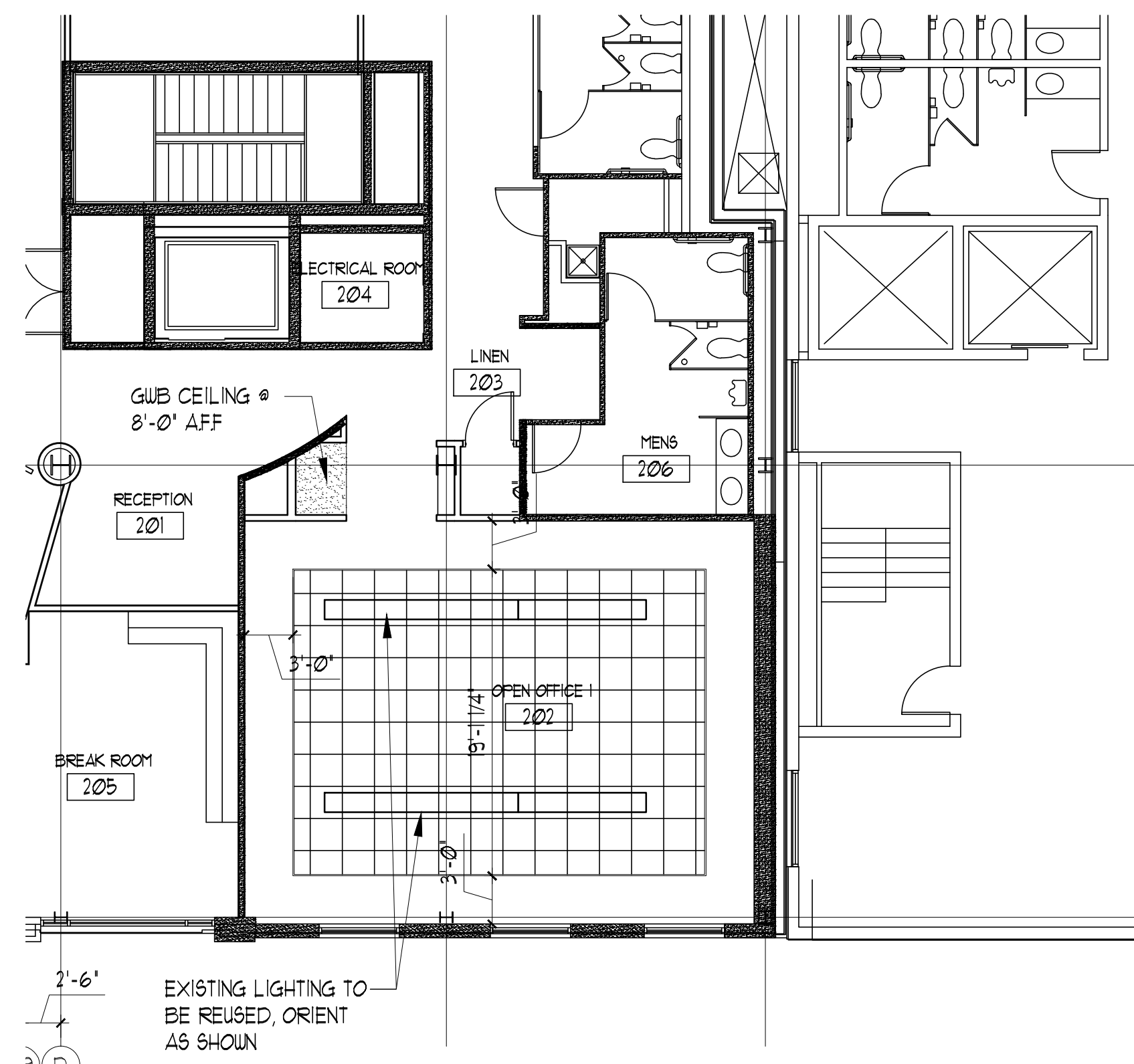
2ND FLOOR PLAN RCP SCALE: 1/8" = 1'-0"
