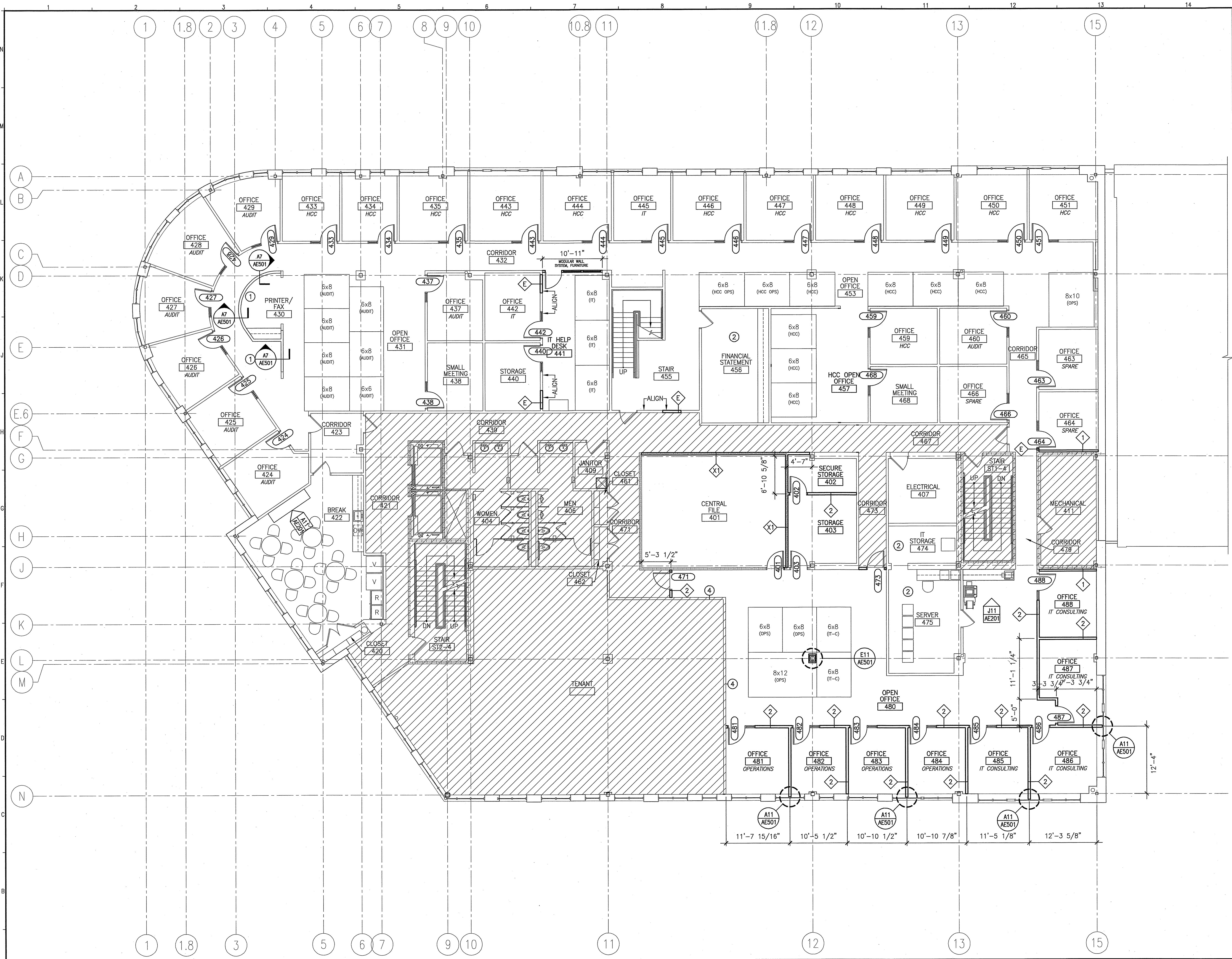
A1 FOURTH LEVEL FLOOR PLAN 1/8" = 1'-0"
