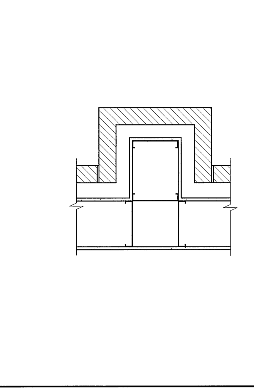
H13 PLAN DETAIL 1"=1'-0"
