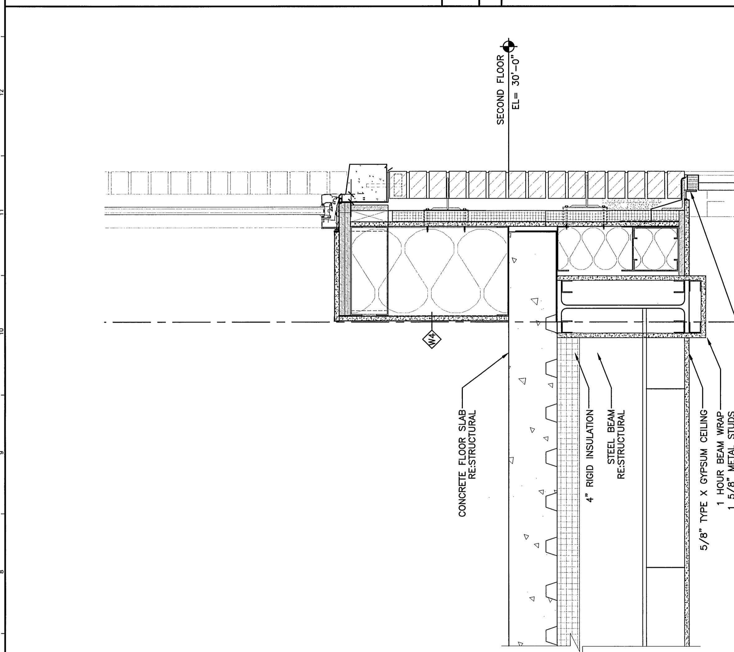
J1 SECTION 1 1/2" = 1'-0"
