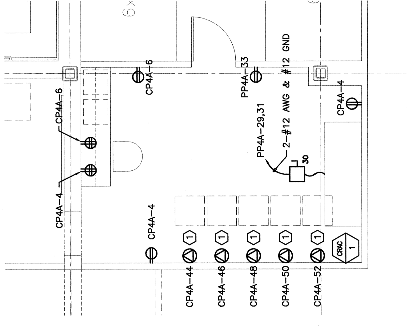
A14 PART PLAN 1/4" = 1'-0"
