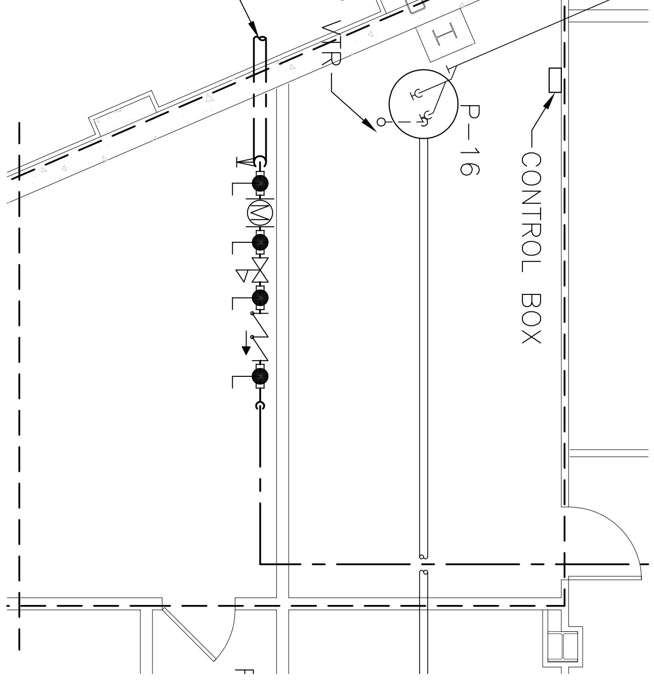
ENLARGED WATER ROOM PLAN SCALE: 1/4" = 1'-0"
