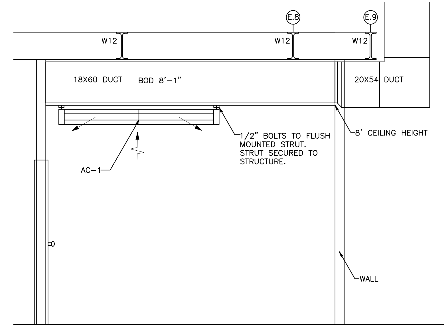
AC-1 MOUNTING DETAIL SCALE: NTS
