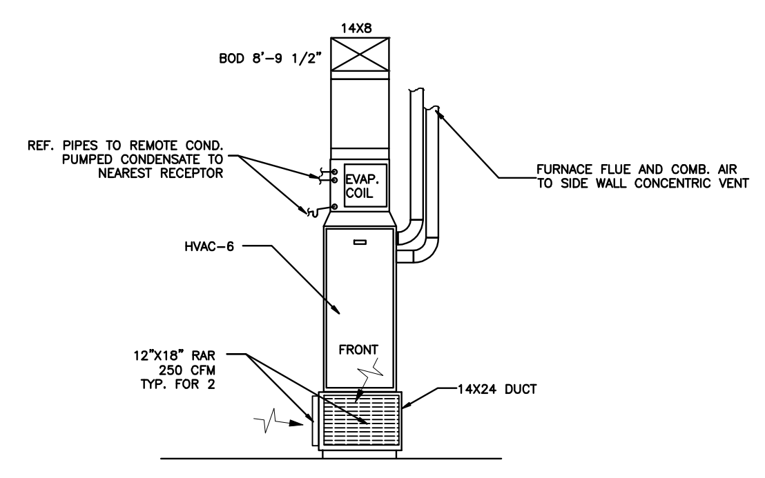
ENLARGED HVAC-6 SCALE: NTS
