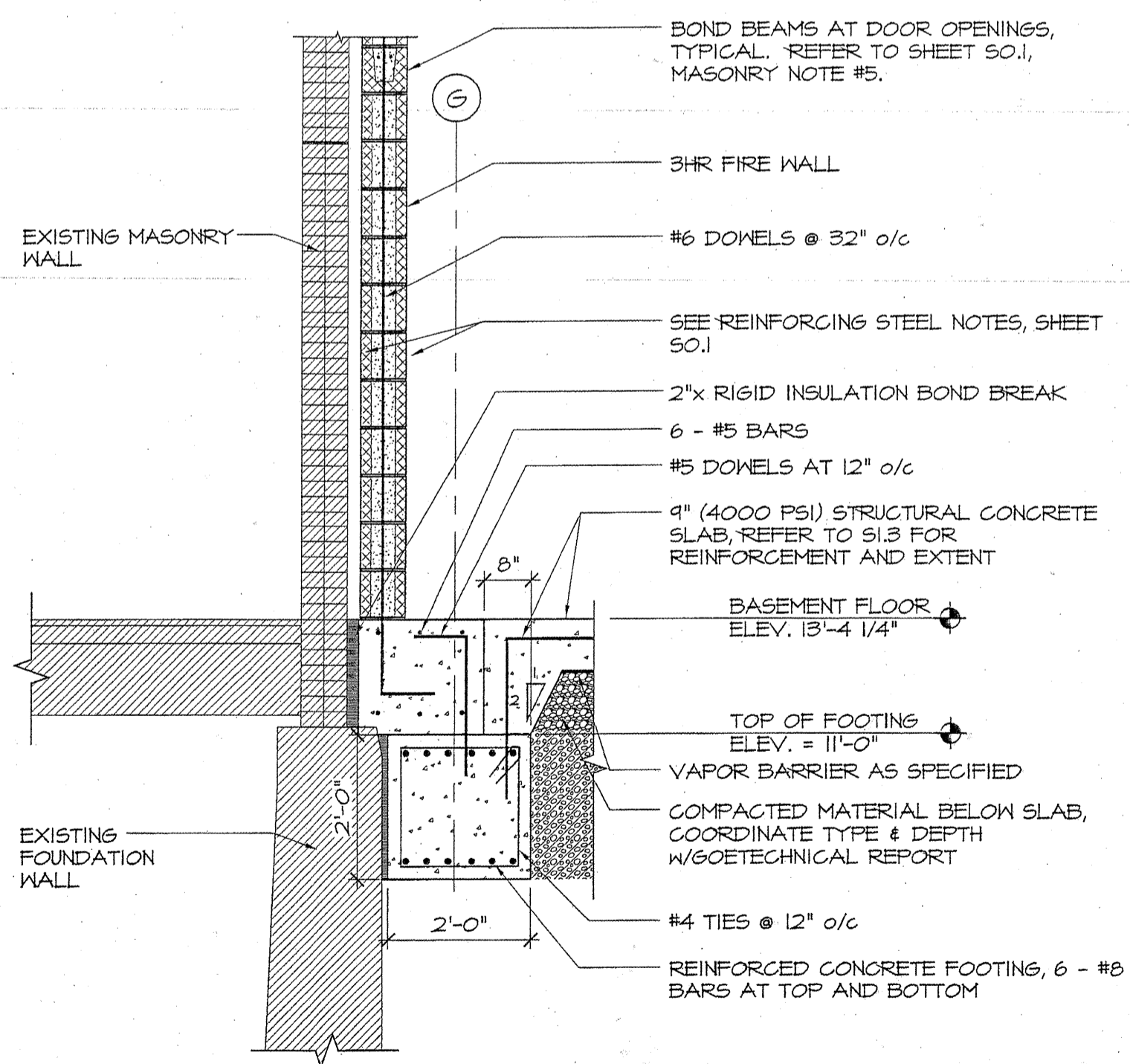
1 FOUNDATION SECTION ALONG 'G' LINE SCALE: 1/2" = 1'-0"
