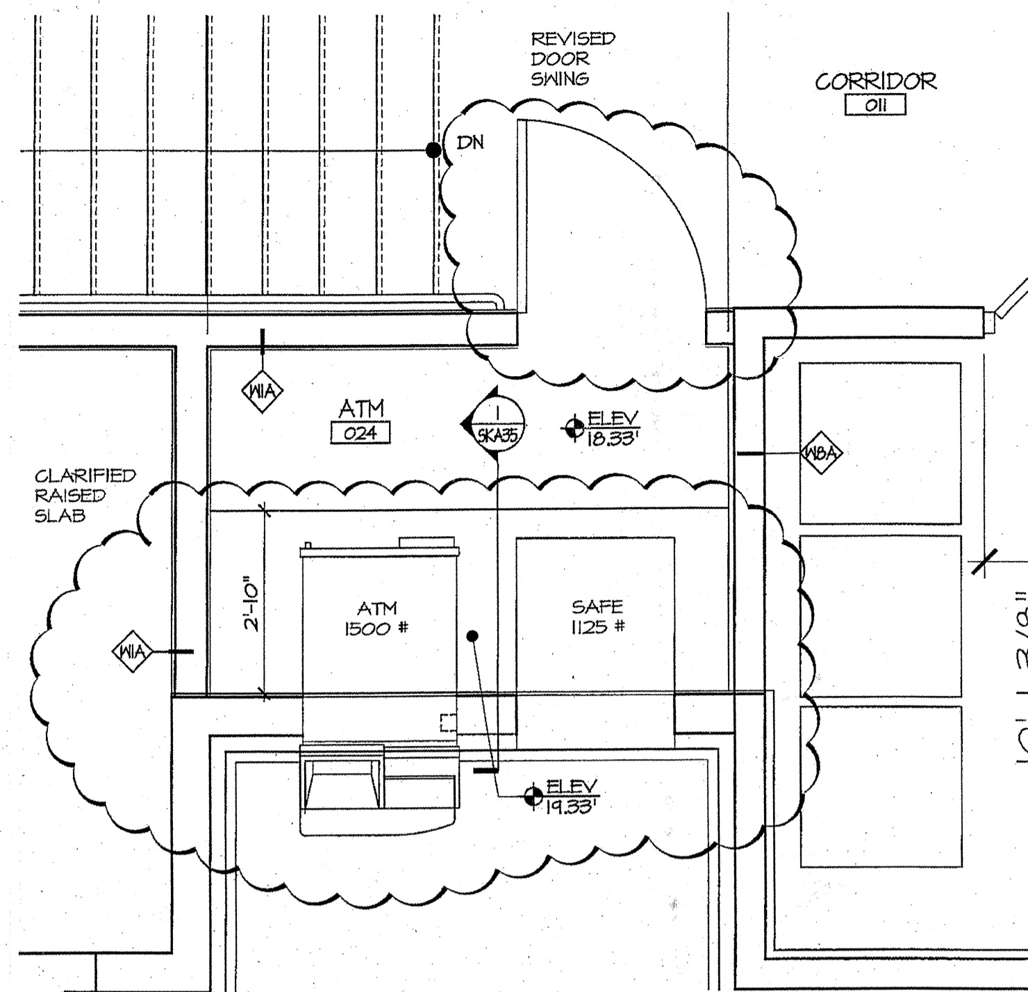
1 ENLARGED ATM ROOM PLAN SCALE: 1/4" = 1'-0"
