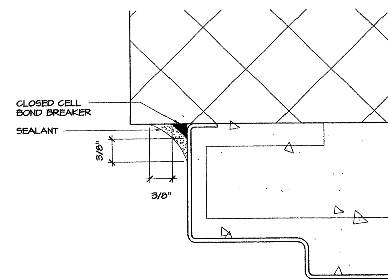
A SEALANT DETAIL AT MASONRY DOOR FRAME SCALE: FULL SCALE
