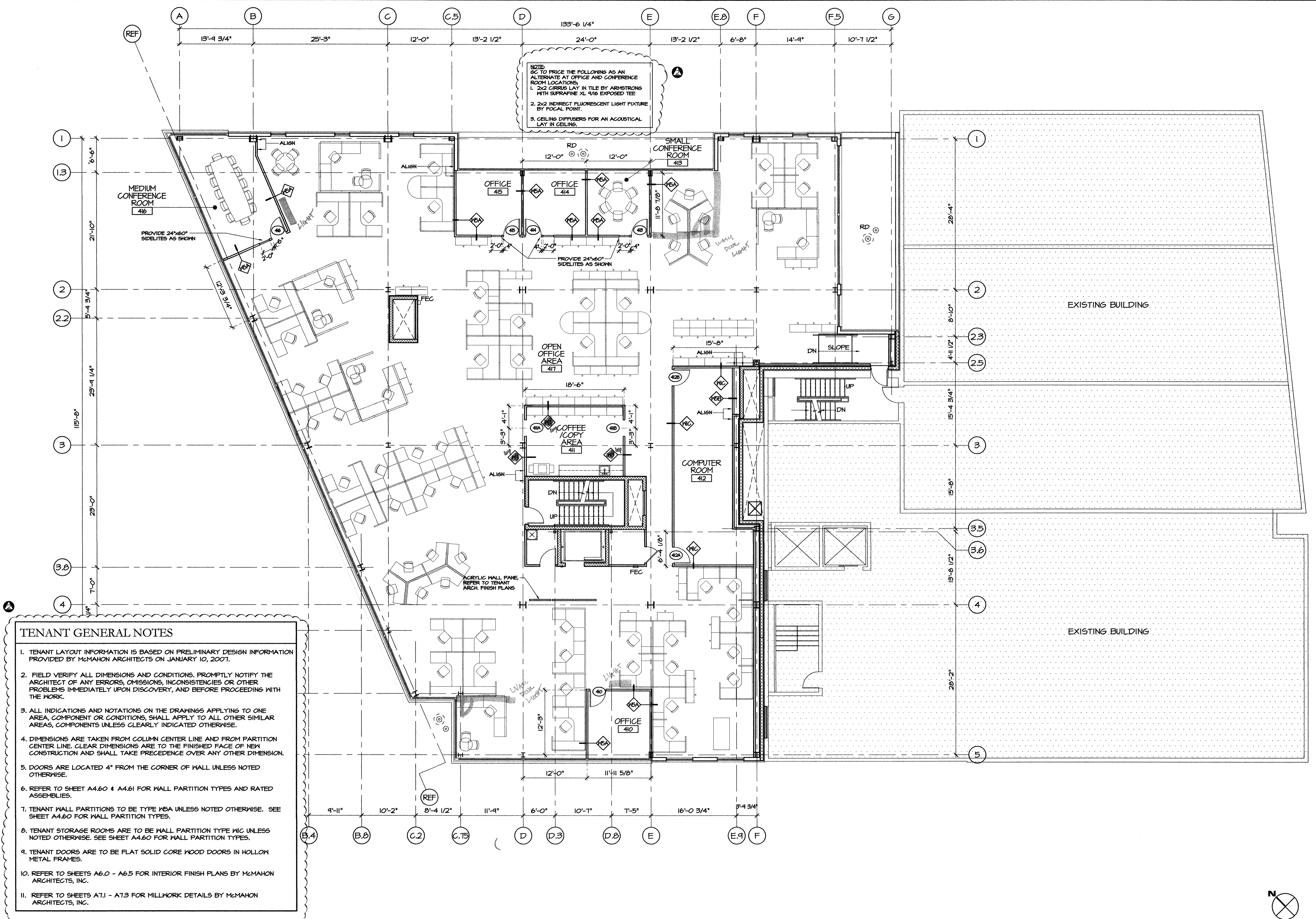
FOURTH FLOOR TENANT FIT-UP PLAN SCALE: 1/8" = 1'-0"
