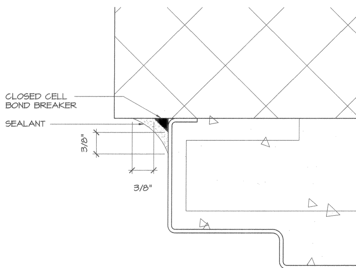
A SEALANT DETAIL AT MASONRY DOOR FRAME SCALE: FULL SCALE
