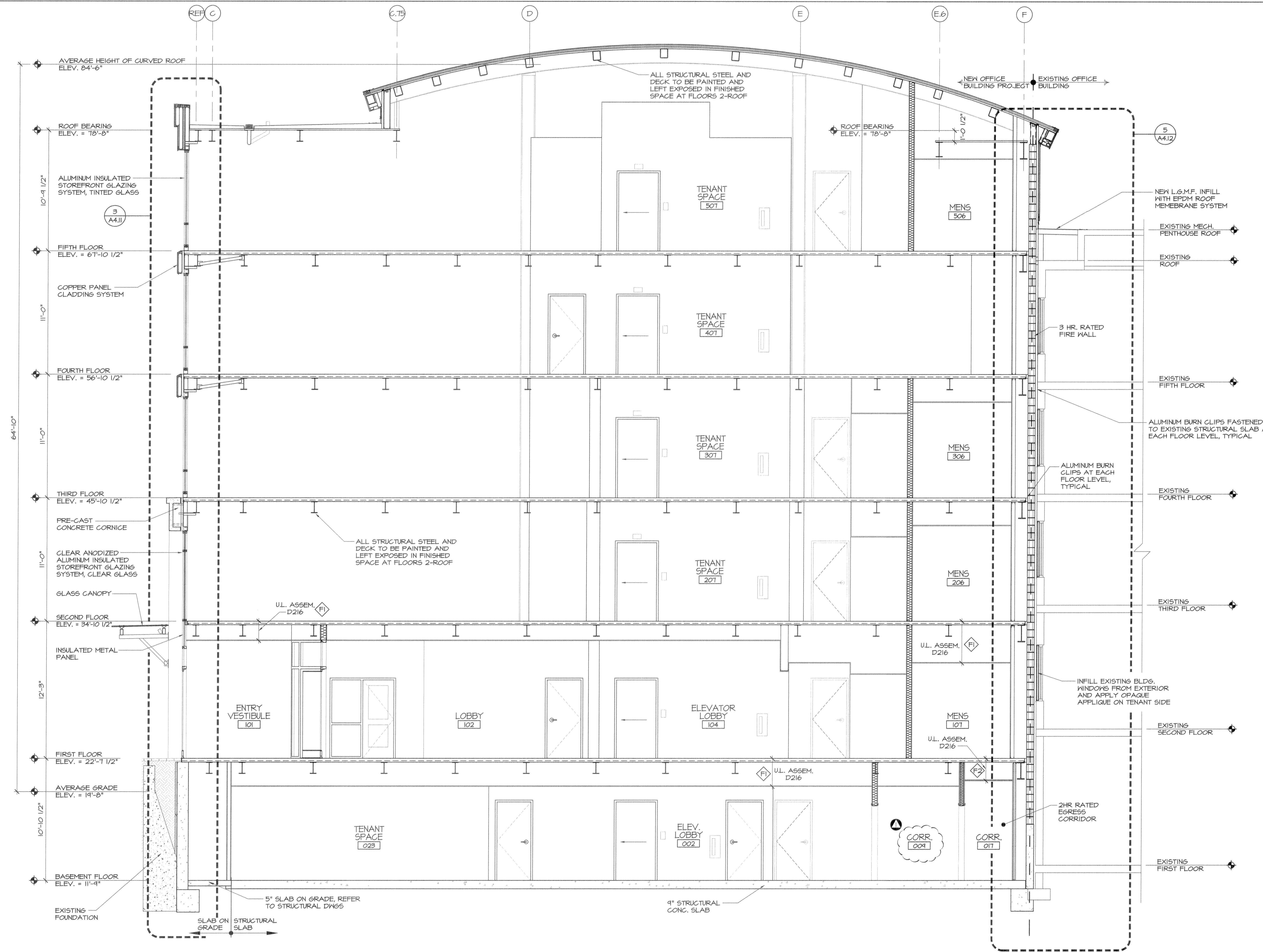
1 BUILDING SECTION SCALE: 1/4" = 1'-0"
