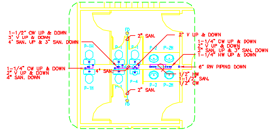
2ND FLOOR PLUMBING DETAIL SCALE 1/4"=1'-0"
