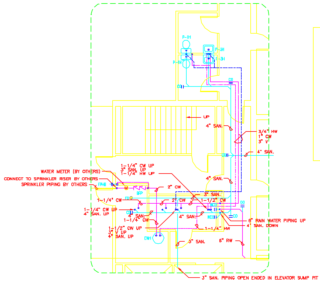
1ST FLOOR PLUMBING DETAIL SCALE 1/4"=1'-0"
