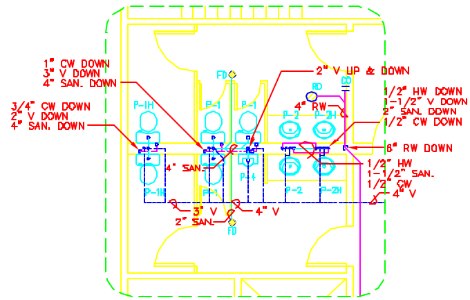
BATHROOM DETAIL SCALE 1/4"=1'-0"
