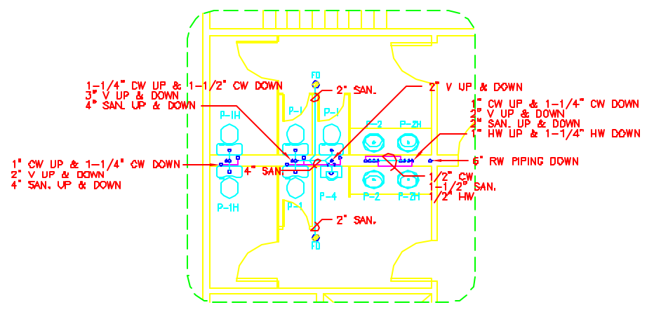
3RD FLOOR PLUMBING PLAN SCALE 1/4"=1'-0"
