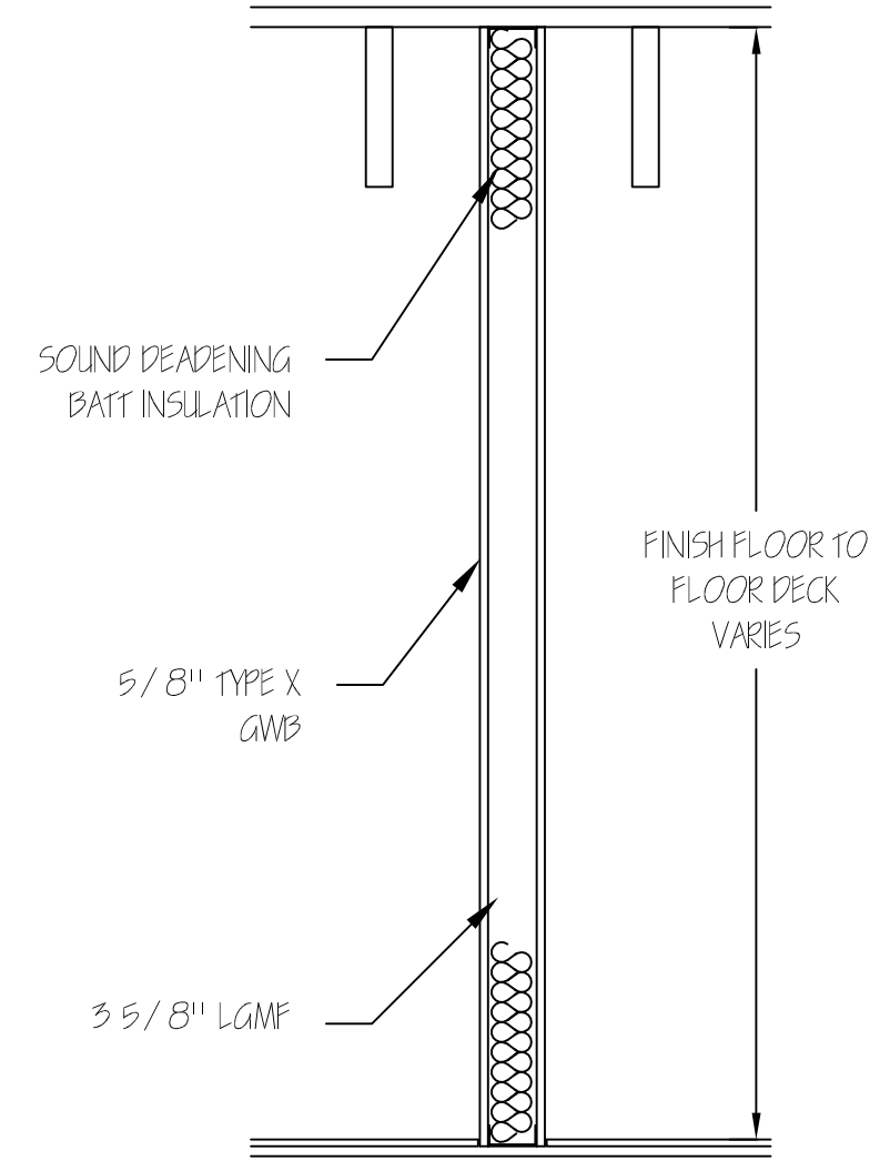
2 TYPICAL WALL SECTION SCALE: 3/4"=1'-0"
