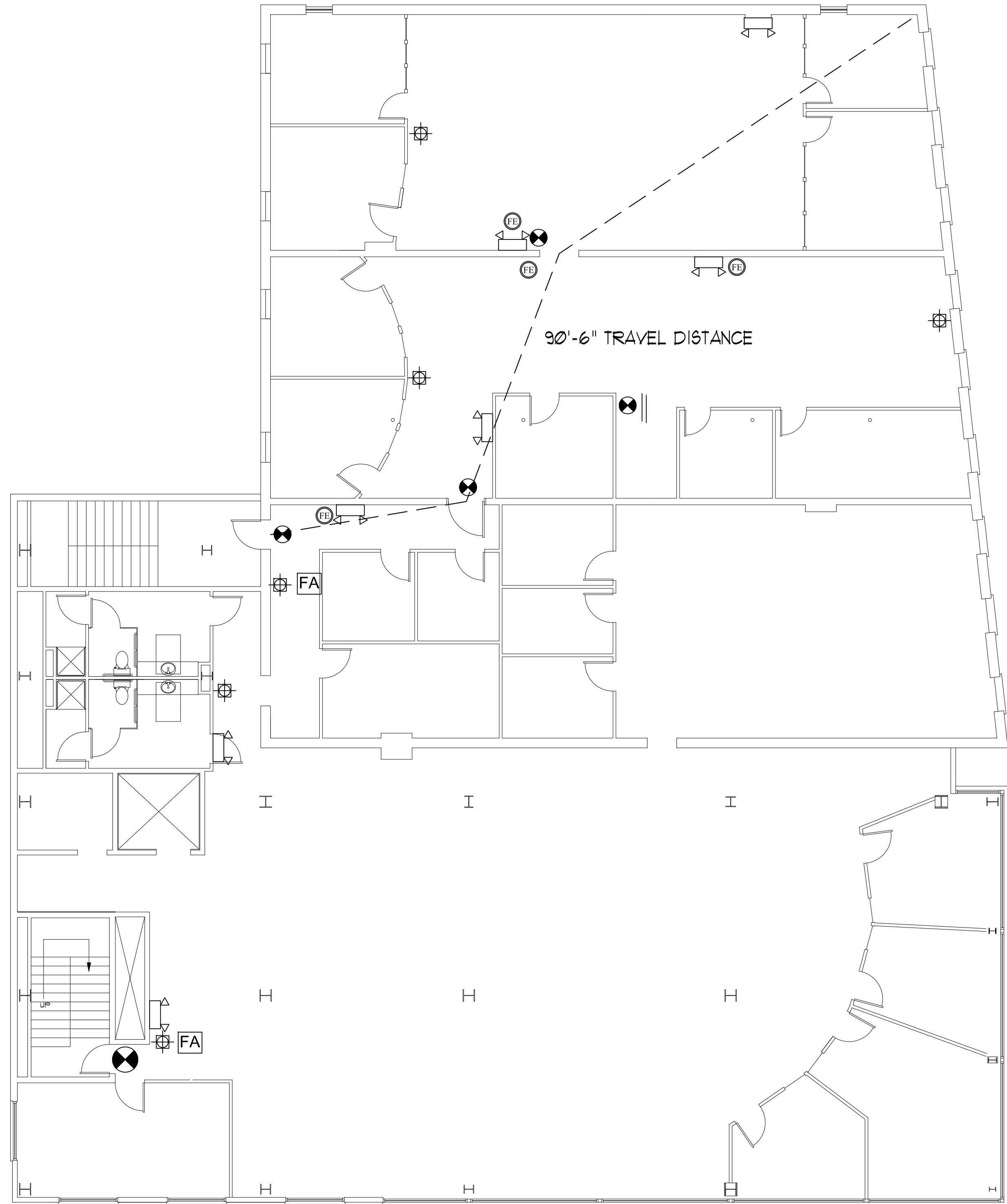
1 | 4th FLOOR LIFE SAFETY PLAN SCALE: 1/8"=1'-0"
