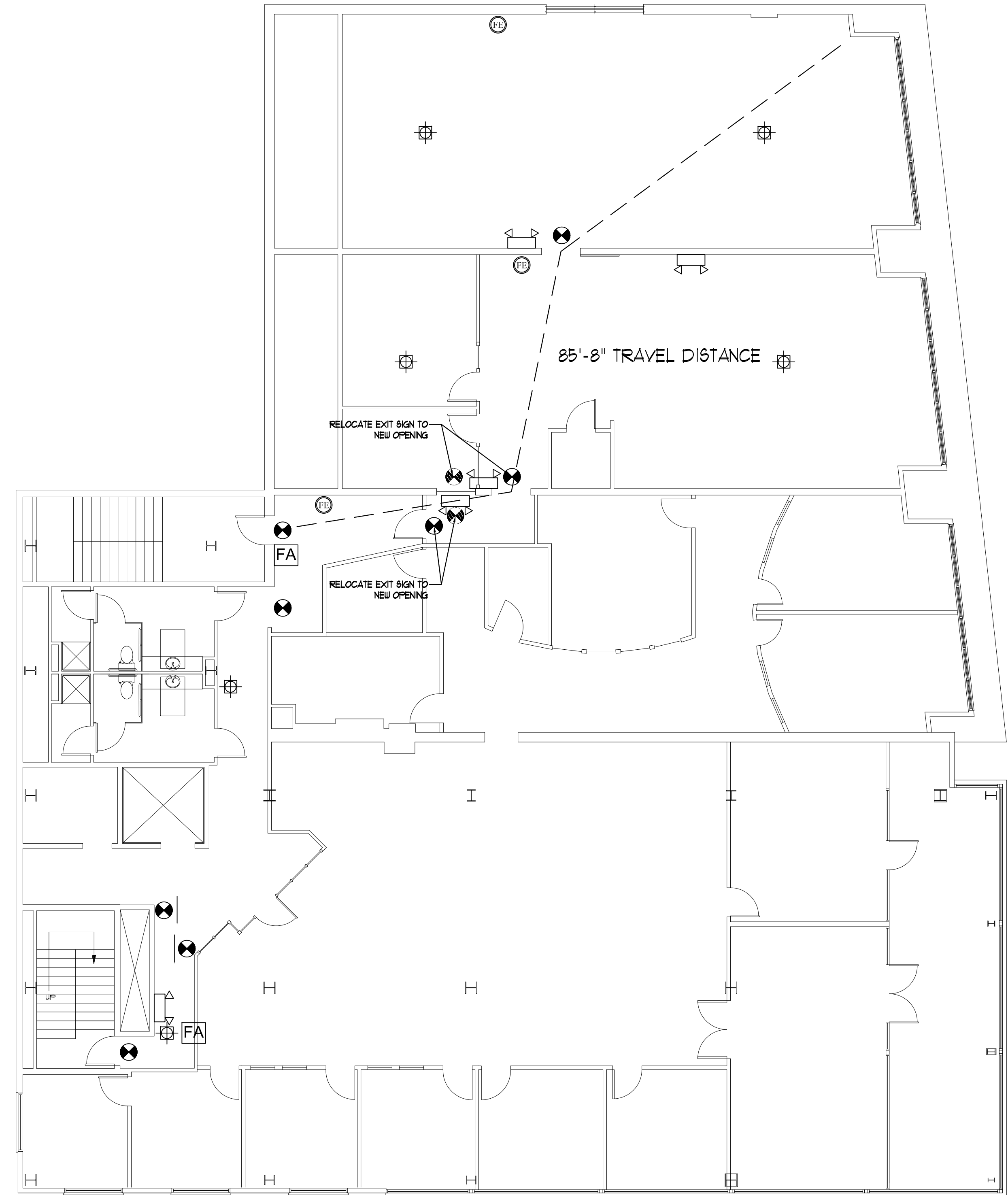
2 | 5th FLOOR LIFE SAFETY PLAN SCALE: 1/8"=1'-0"
