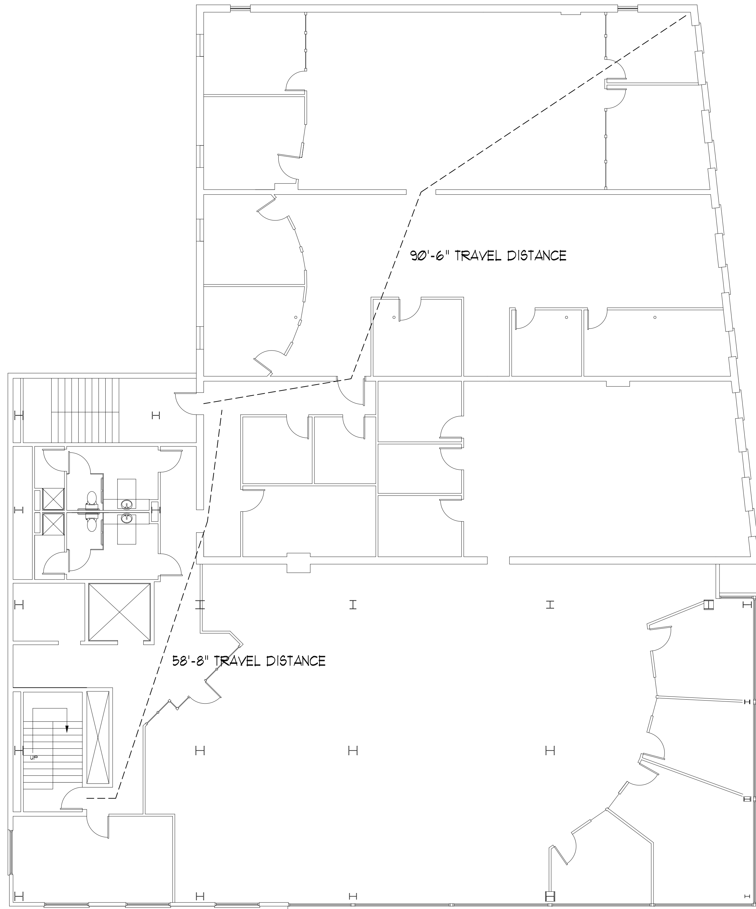
1 | 4th FLOOR LIFE SAFETY PLAN SCALE: 1/8"=1'-0"
