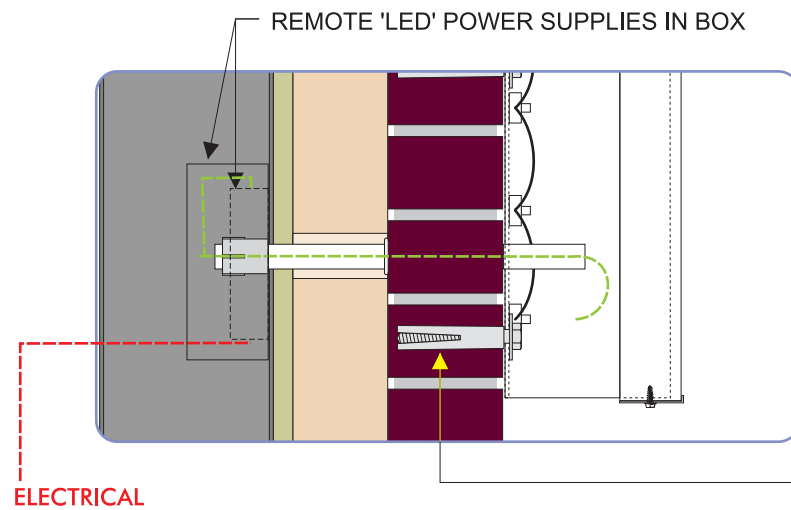
SIMILAR WALL/FABRICATION - DETAILS (TBD)
