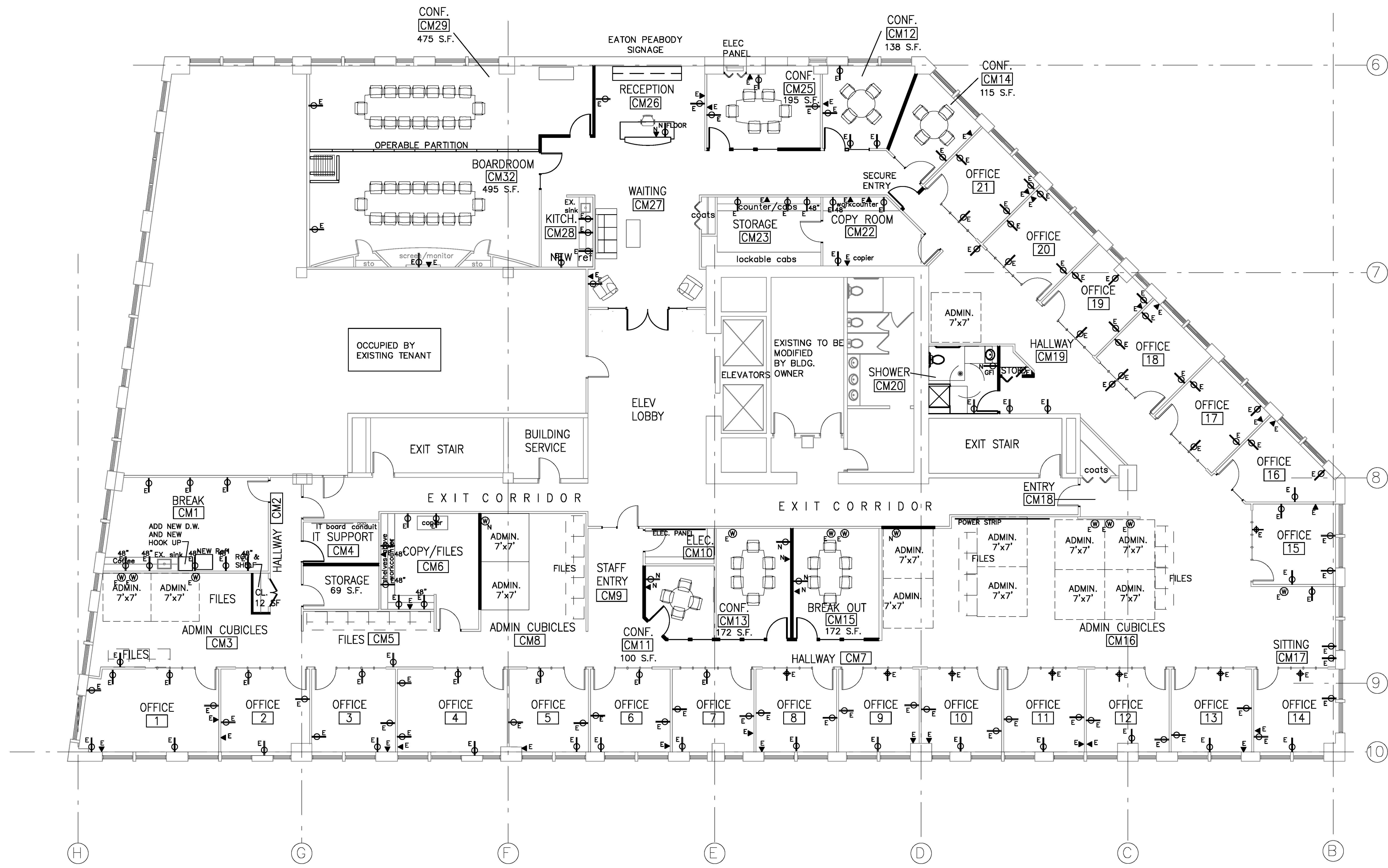
AI SECOND FLOOR POWER PLAN 1/8"=1'-0"
