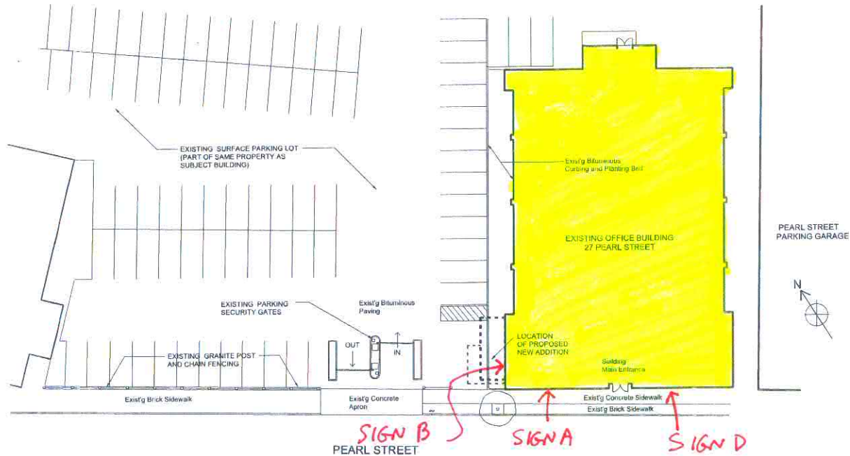
1 EXISTING CONDITIONS SITE PLAN scale: 1/16" = 1'-0"
