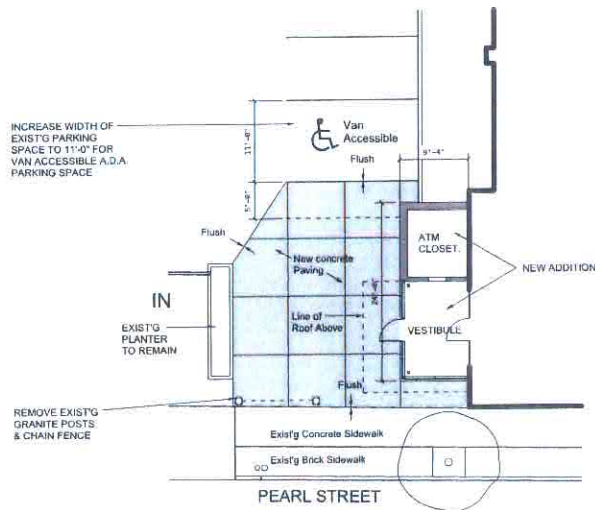
2 PROPOSED CONDITIONS SITE PLAN scale: 1/8" = 1'-0"
