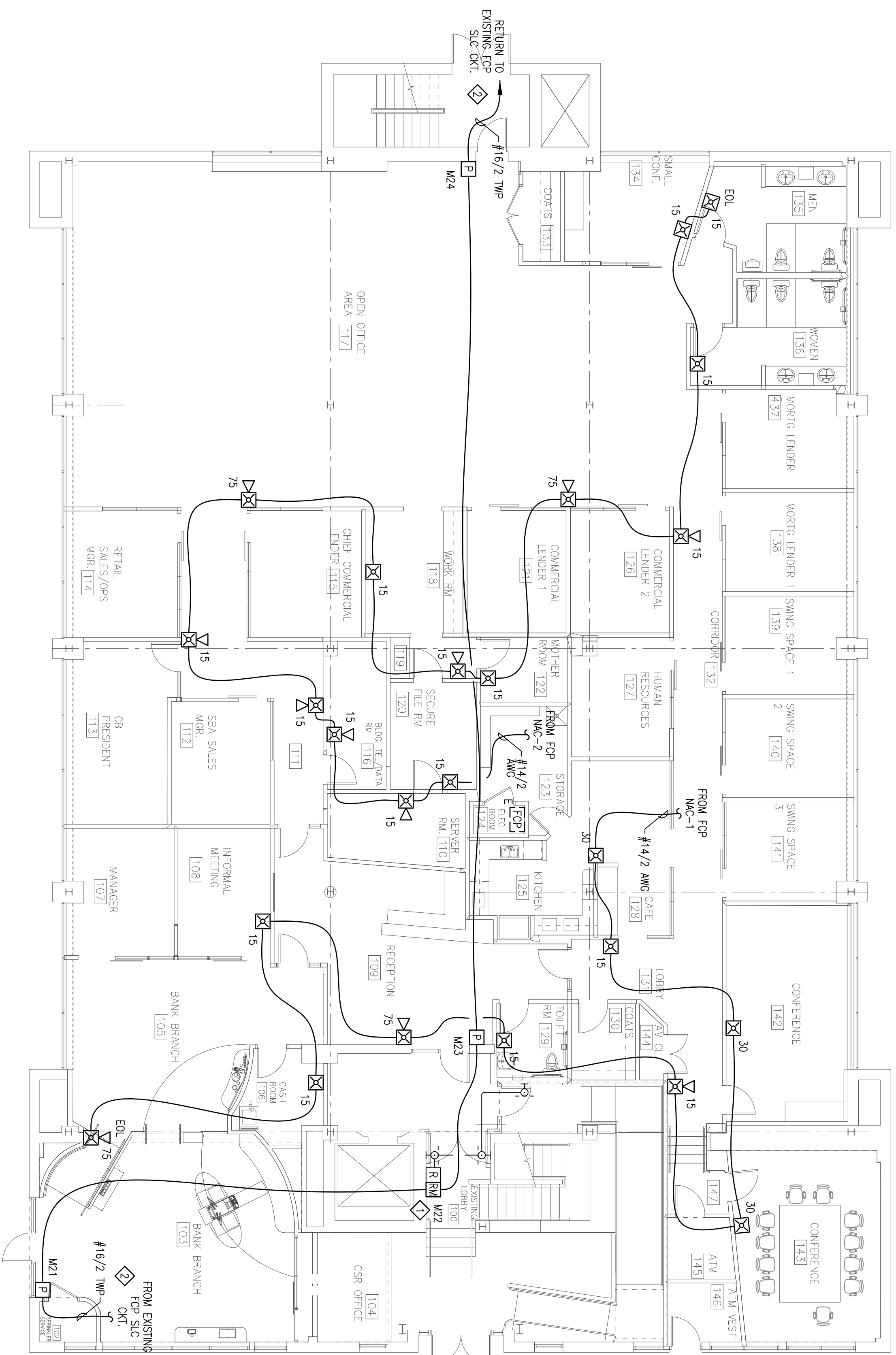
FIRST FLOOR TENANT IMPROVEMENT FIRE ALARM PLAN SCALE: 1/8"=1'-0"
