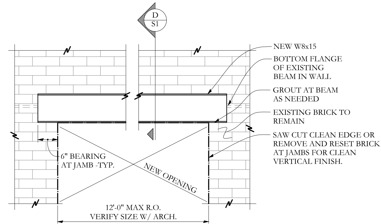
TYP. ELEVATION B S3.1 3/4"=1'-0
