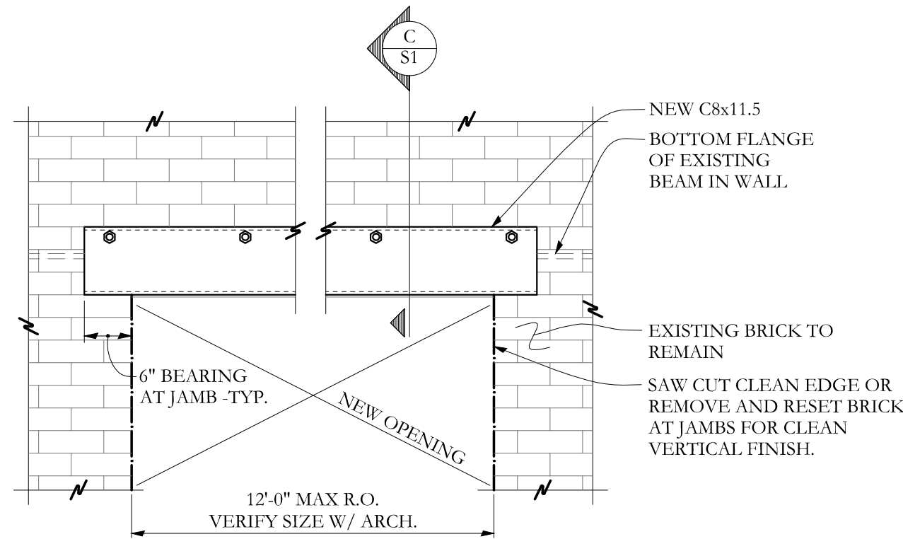
TYP. ELEVATION A S3.1 3/4"=1'-0
