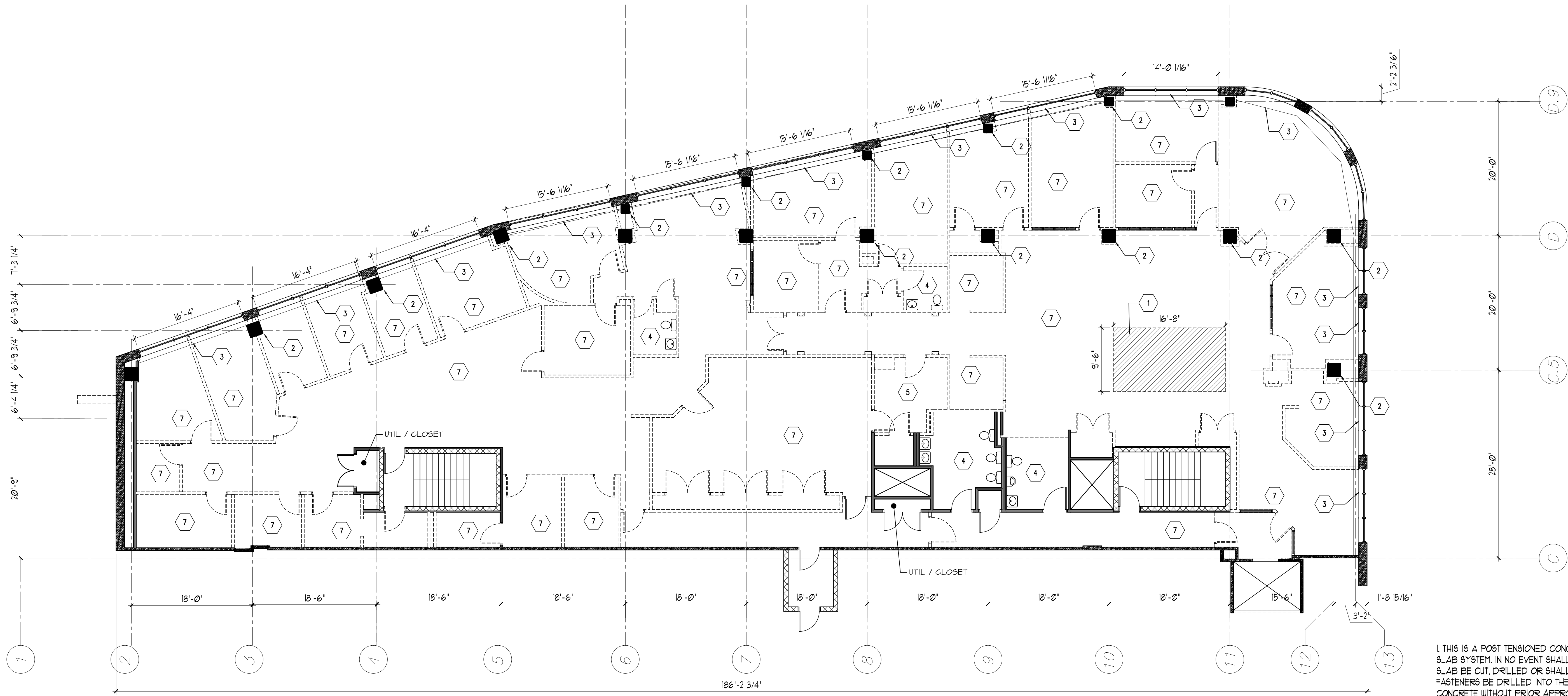
3RD FLOOR - DEMO PLAN SCALE: 1/8" = 1'-0"
