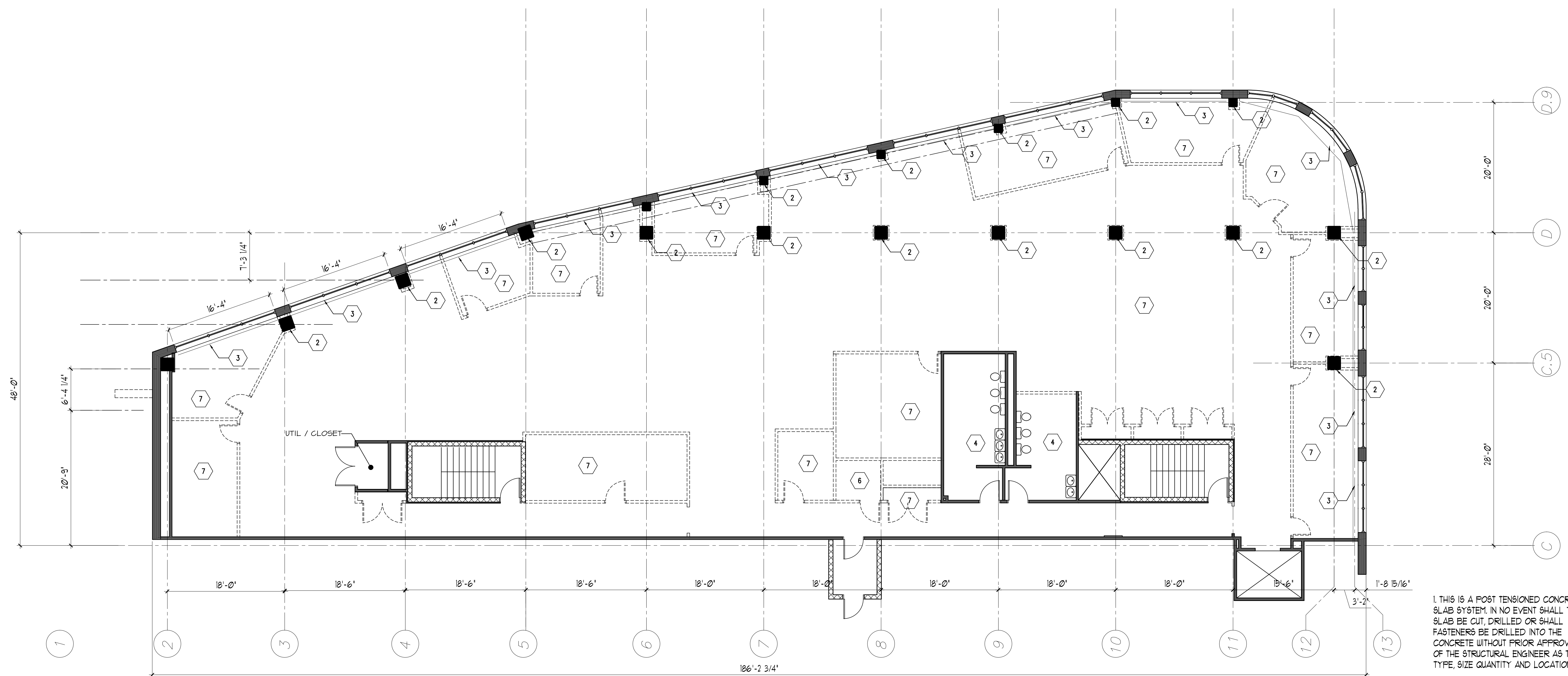
2ND FLOOR - DEMO PLAN SCALE: 1/8" = 1'-0"
