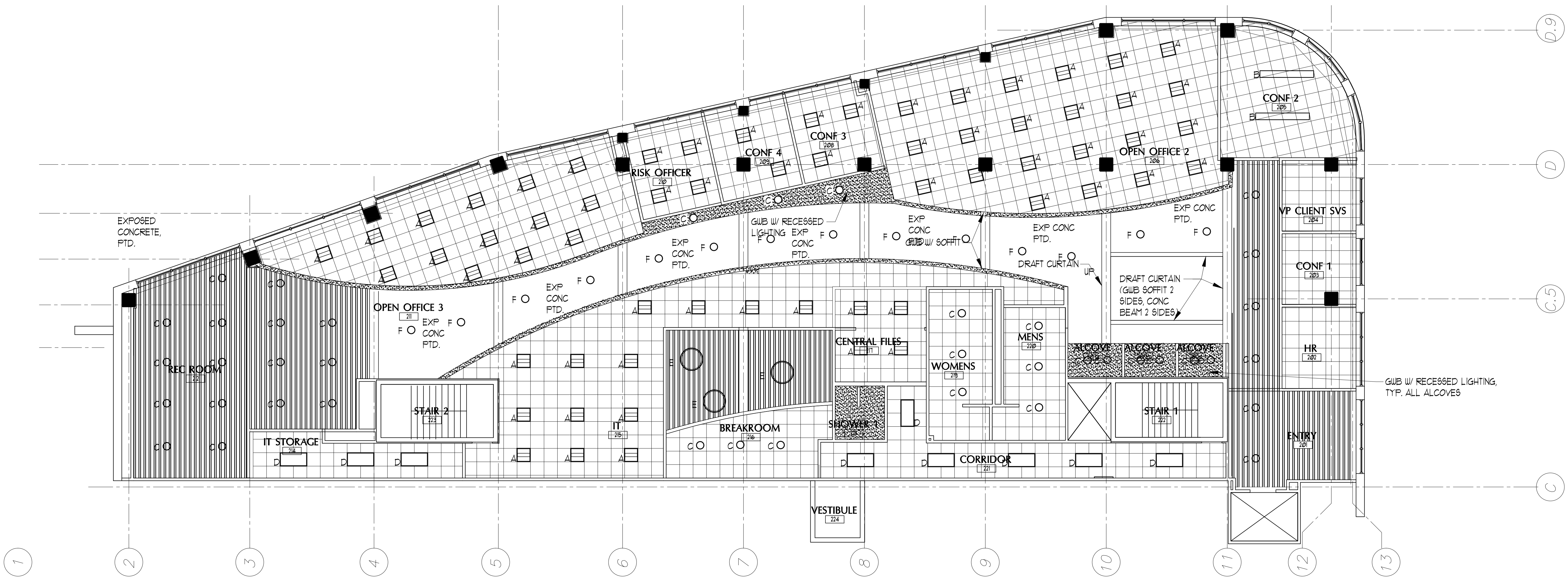
2ND FLOOR RCP SCALE: 1/8" = 1'-0"
