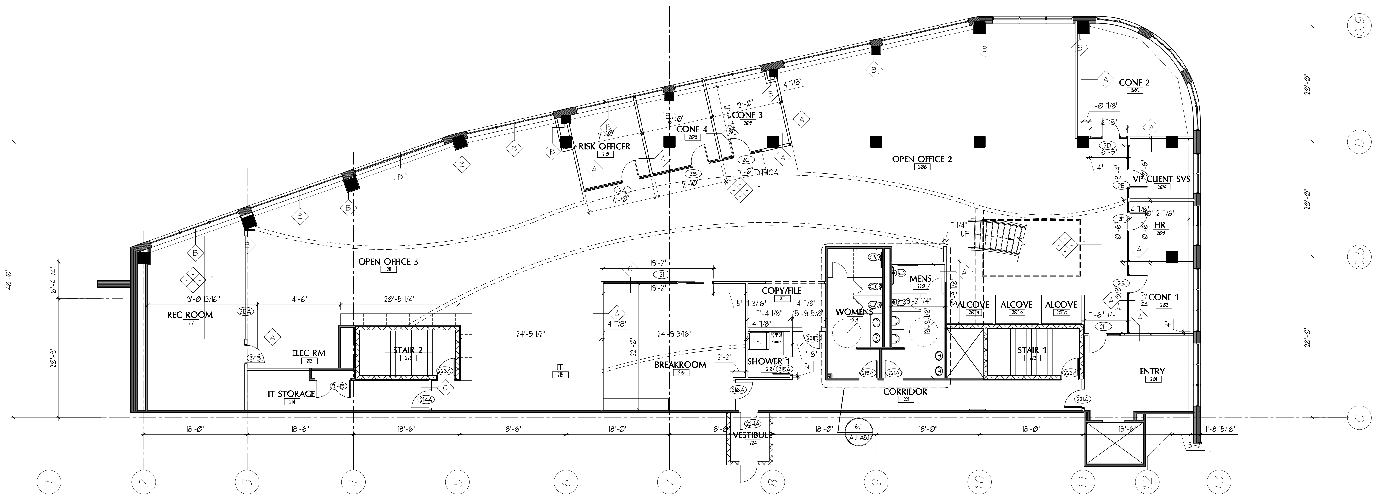
1 2ND FLOOR PLAN SCALE: 1/8" = 1'-0"
