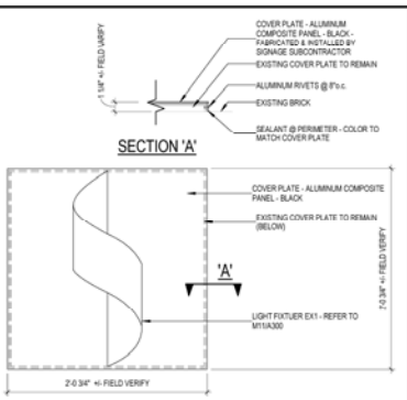
2 EX1 - EXTERIOR SCONCE
