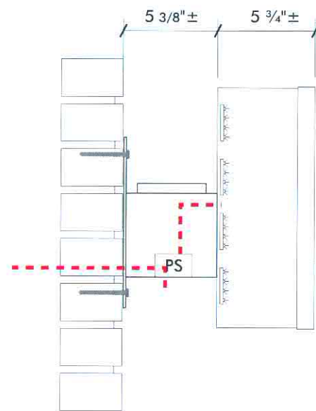
SECTION - (TYPICAL) SCALE: 1 1/2" = 1'-0"
