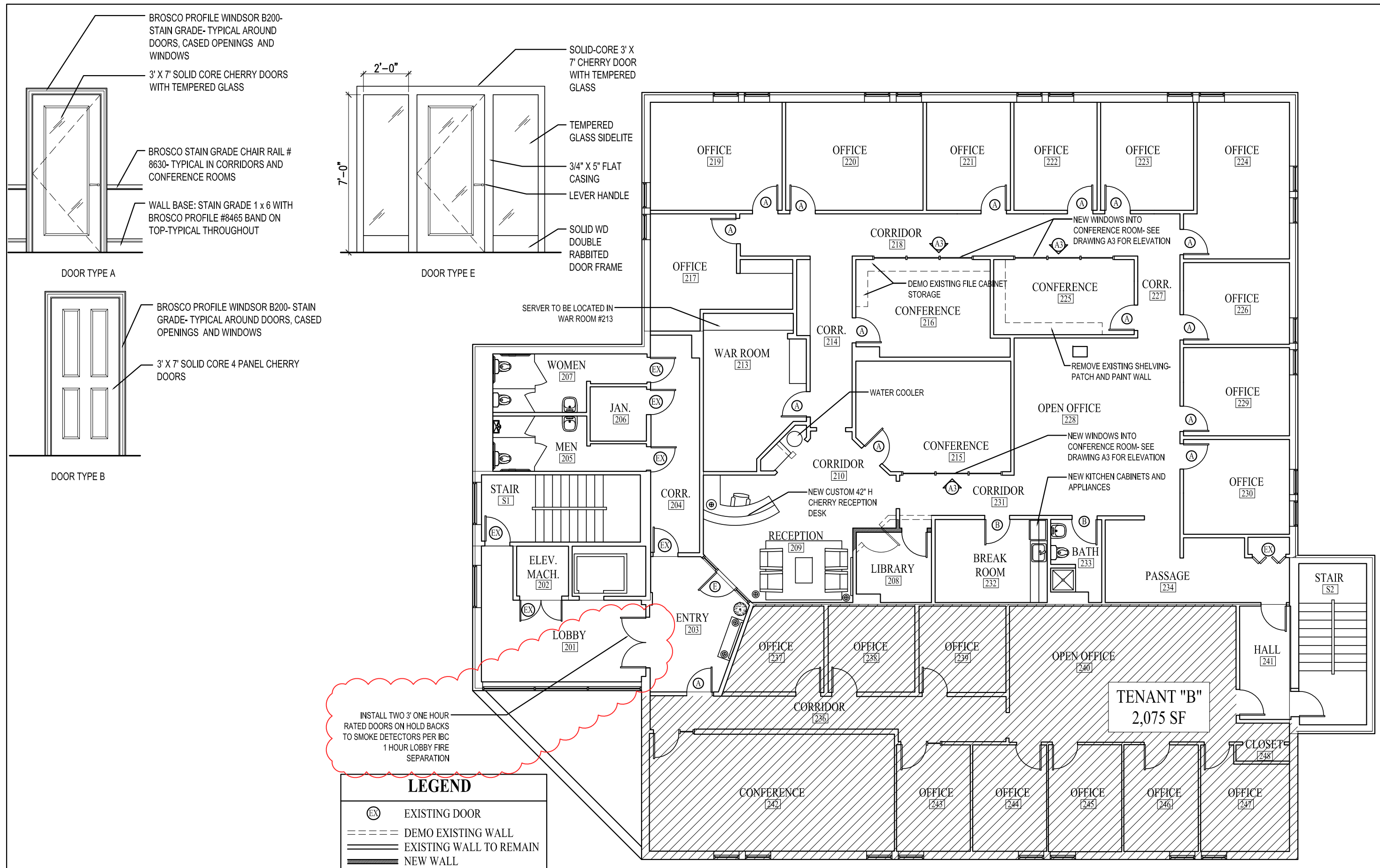
1 | FLOOR PLAN- SECOND FLOOR SCALE: 3/32"=1'-0"
