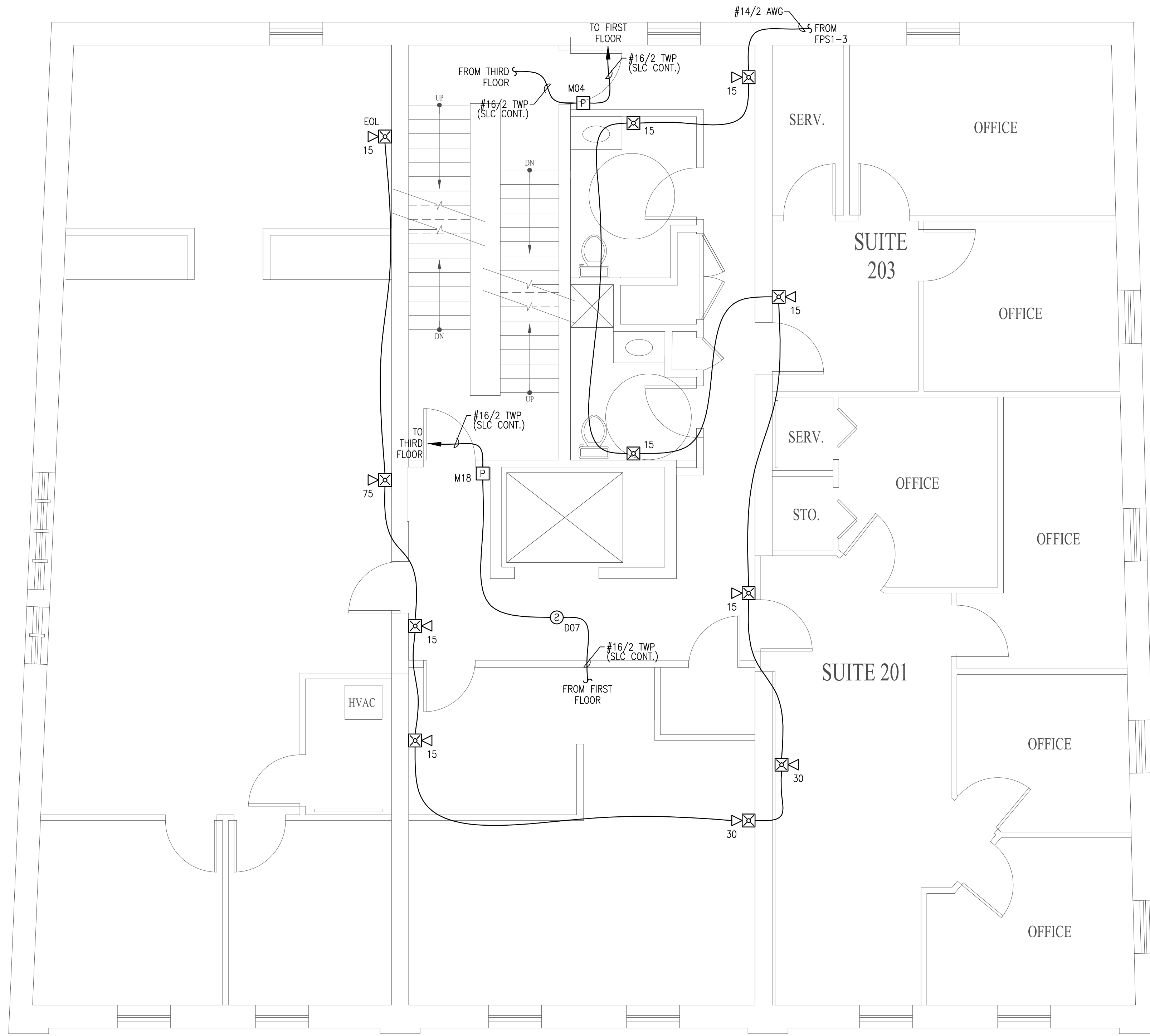
PLAN NORTH SECOND FLOOR FIRE ALARM PLAN SCALE: 1/4"=1'-0"
