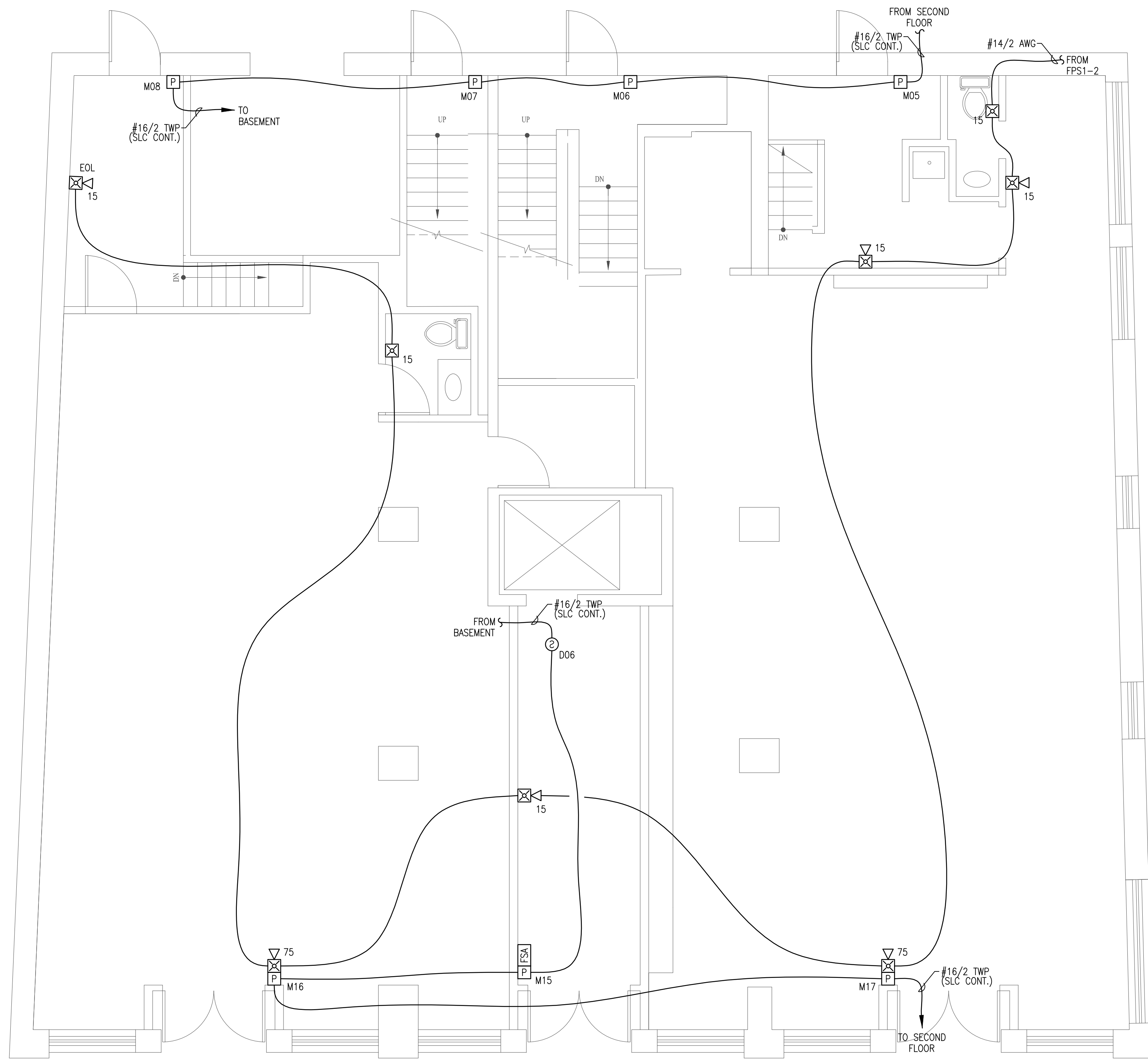
PLAN NORTH FIRST FLOOR FIRE ALARM PLAN SCALE: 1/4"=1'-0"
