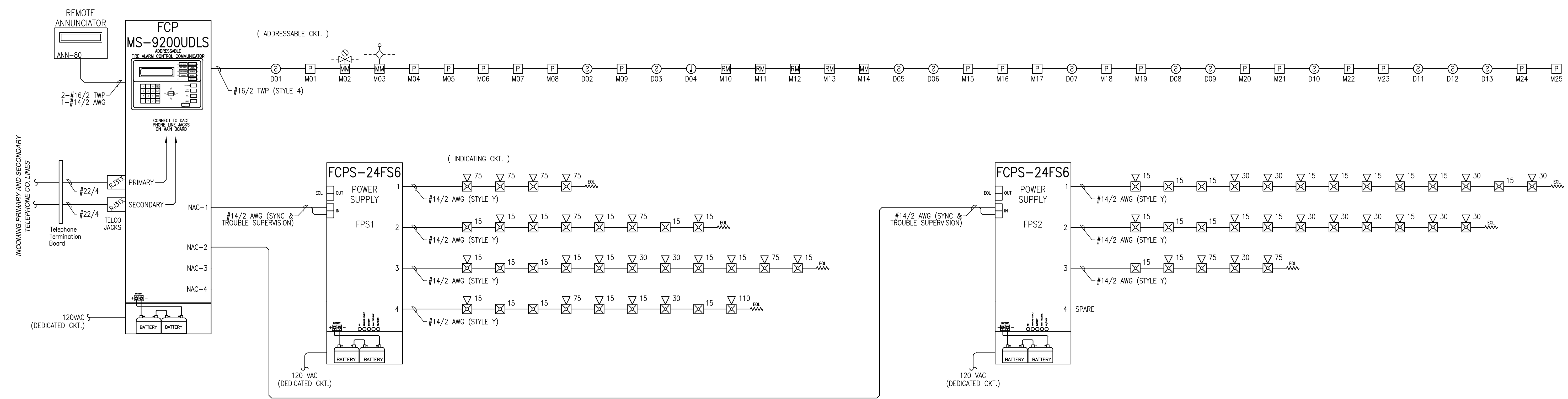
FIRE ALARM RISER DIAGRAM SCHEMATIC: NO SCALE
