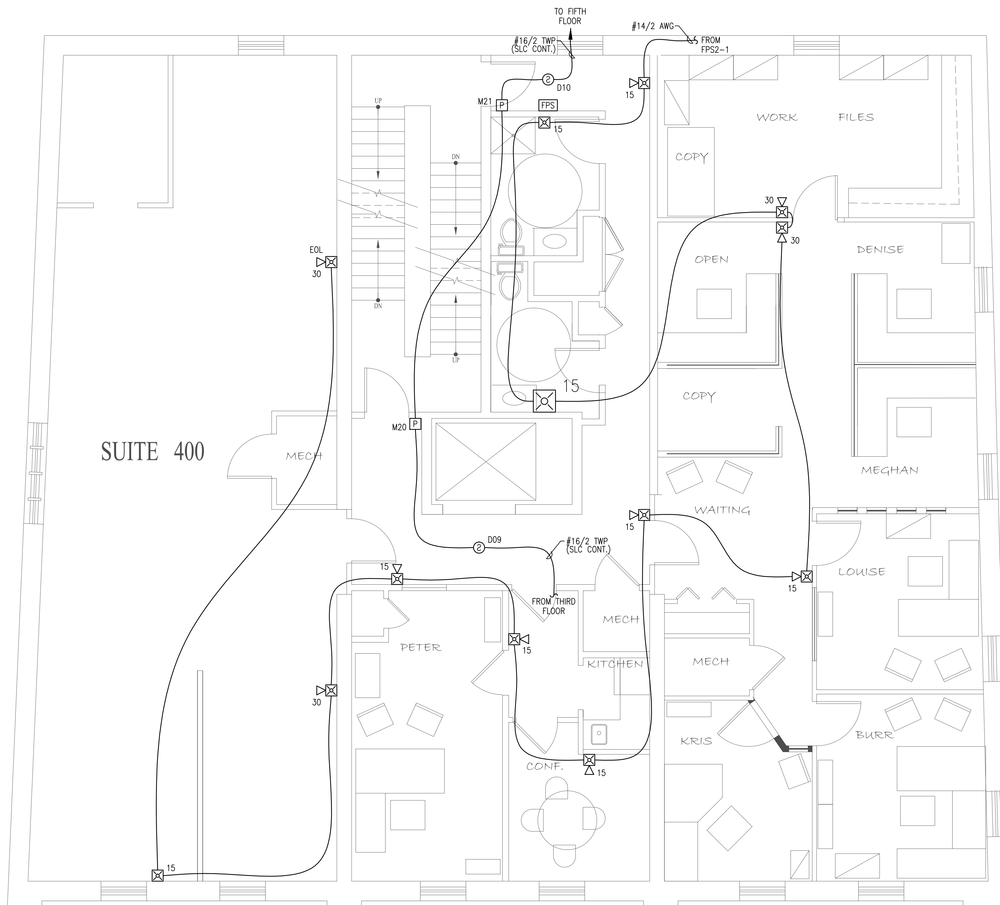
PLAN NORTH FOURTH FLOOR FIRE ALARM PLAN SCALE: 1/8"=1'-0"
