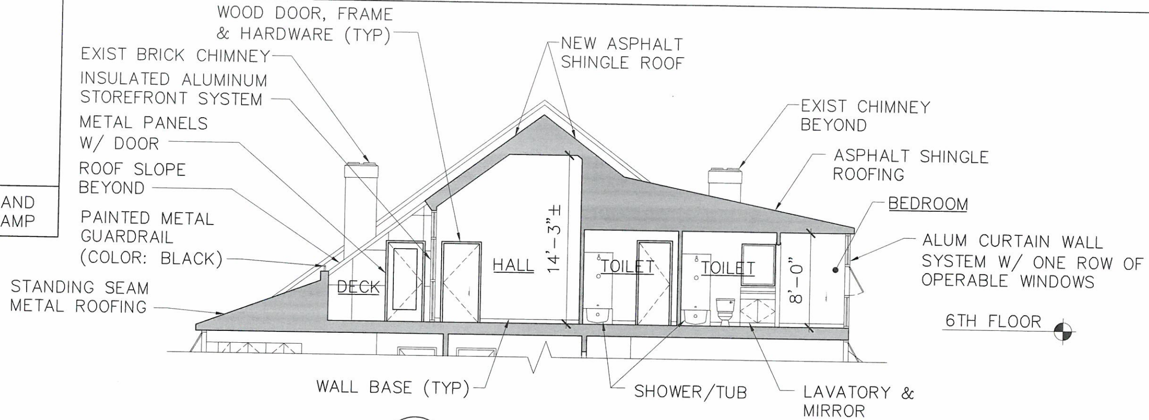
1 PARTIAL BLDG SECTION SKA1 SCALE: 1/8"=1'-0"
