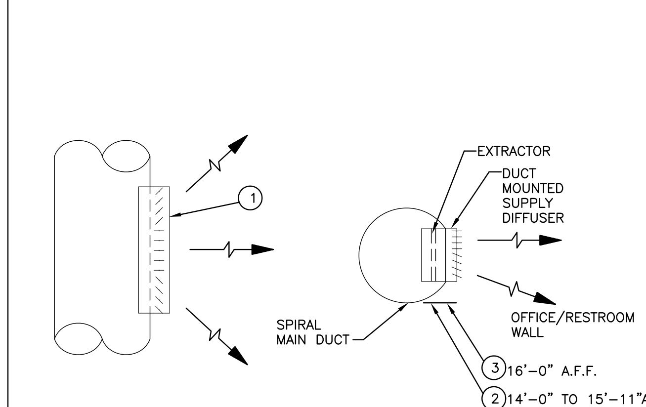
DIFFUSER MOUNTING DETAIL NOT TO SCALE 103
