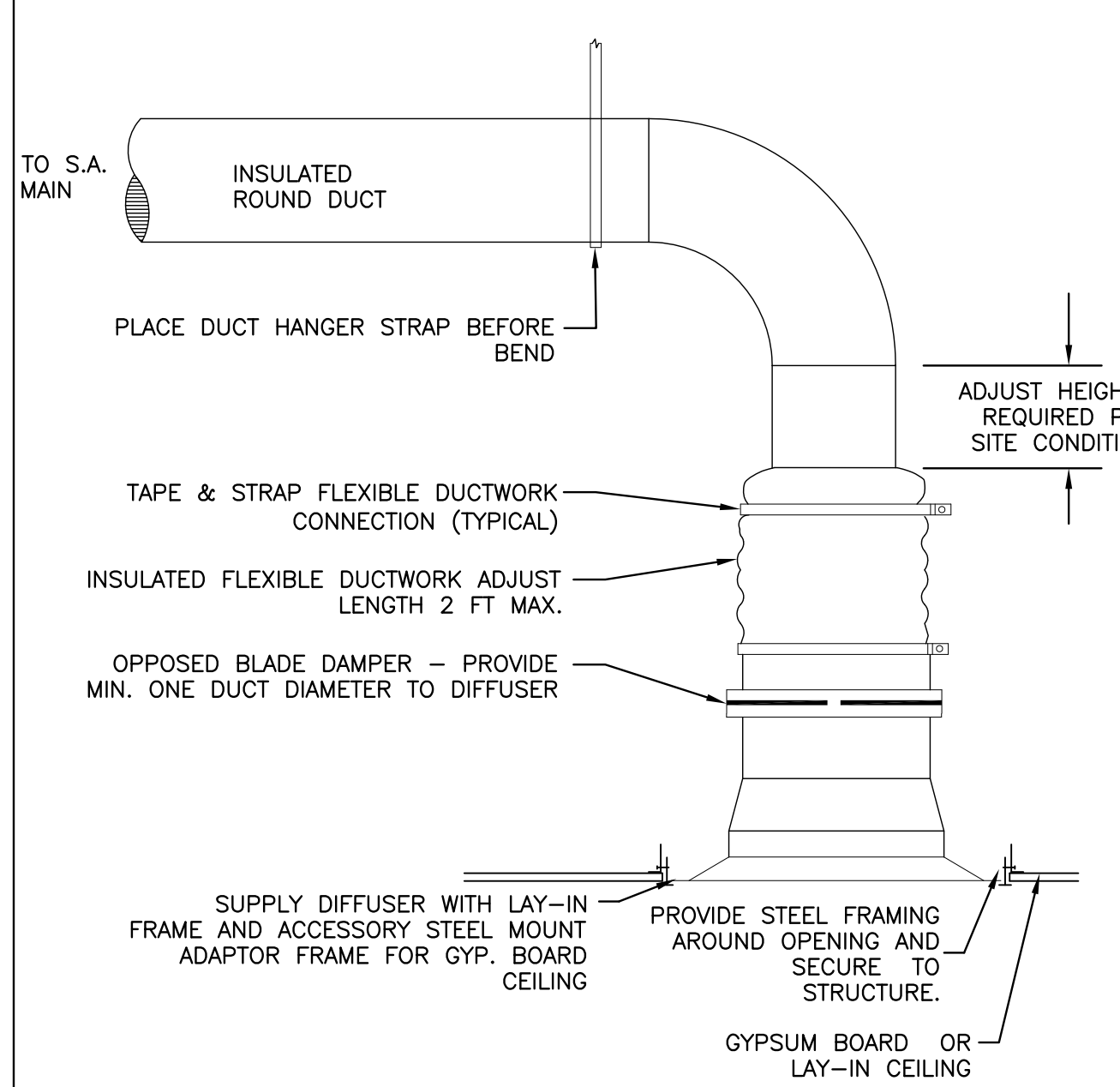
DIFFUSER MOUNTING DETAIL NOT TO SCALE 103
