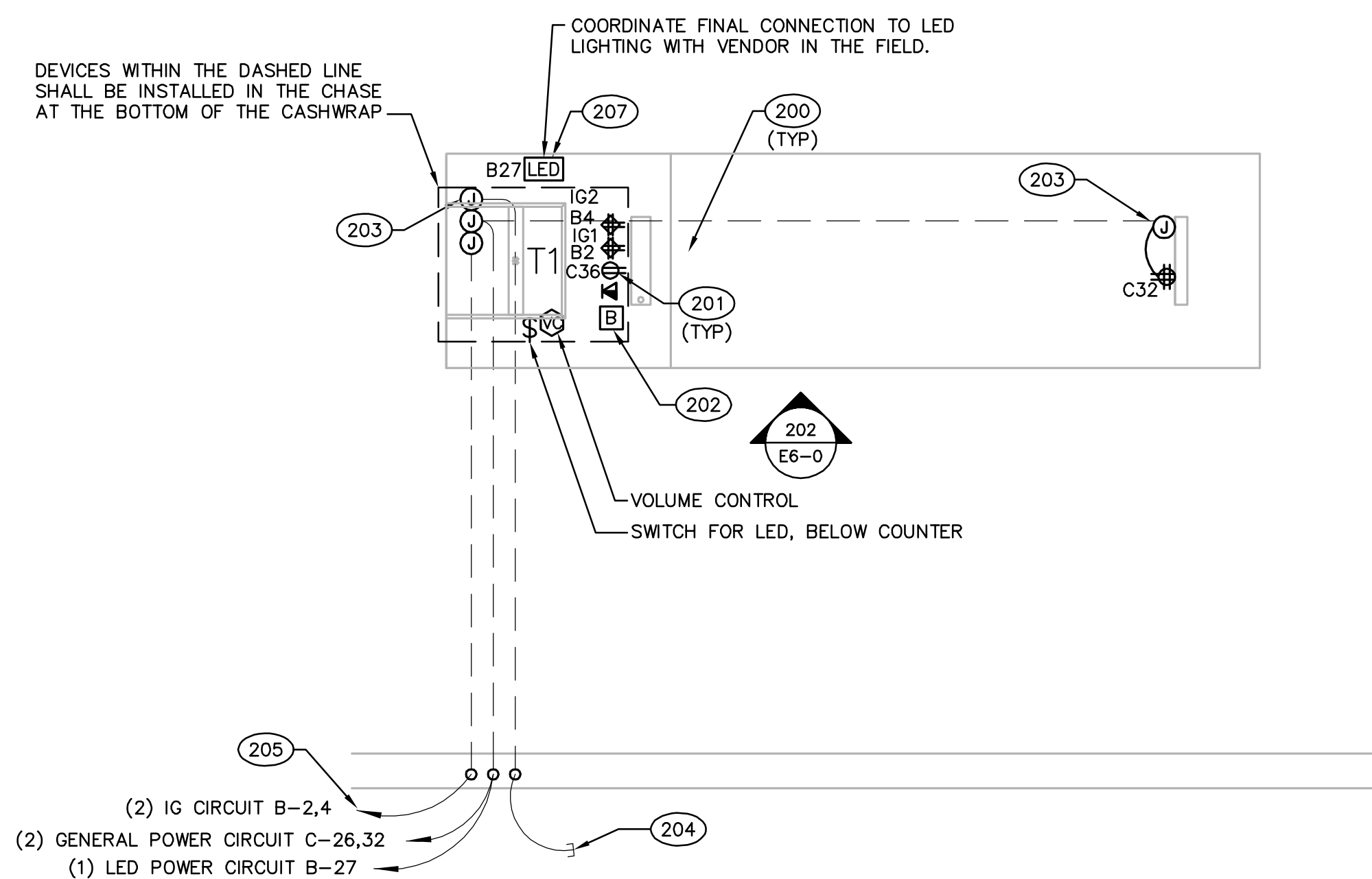
1-TERMINAL CASHWRAP PLAN LAYOUT
