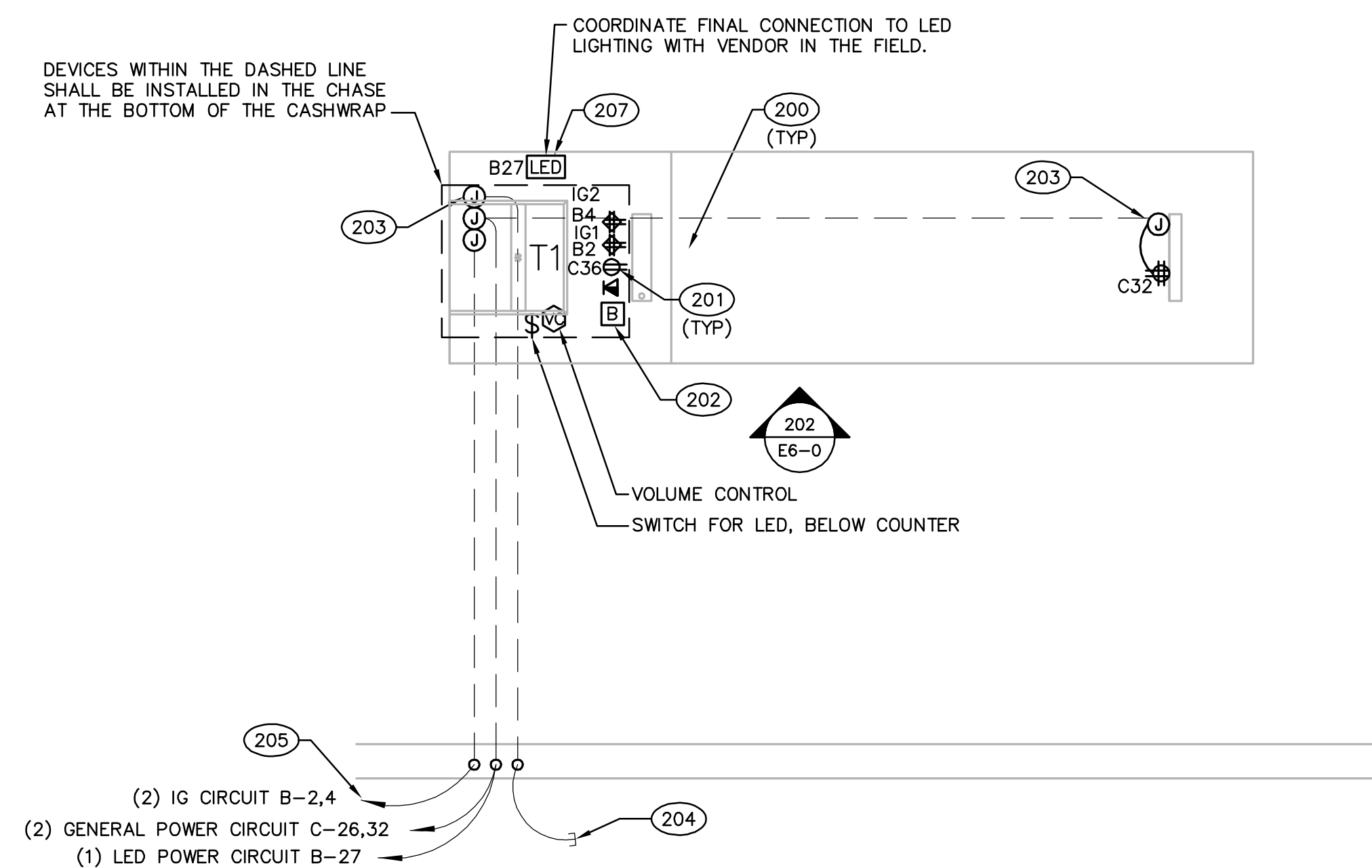
1-TERMINAL CASHWRAP ELEVATION LAYOUT
