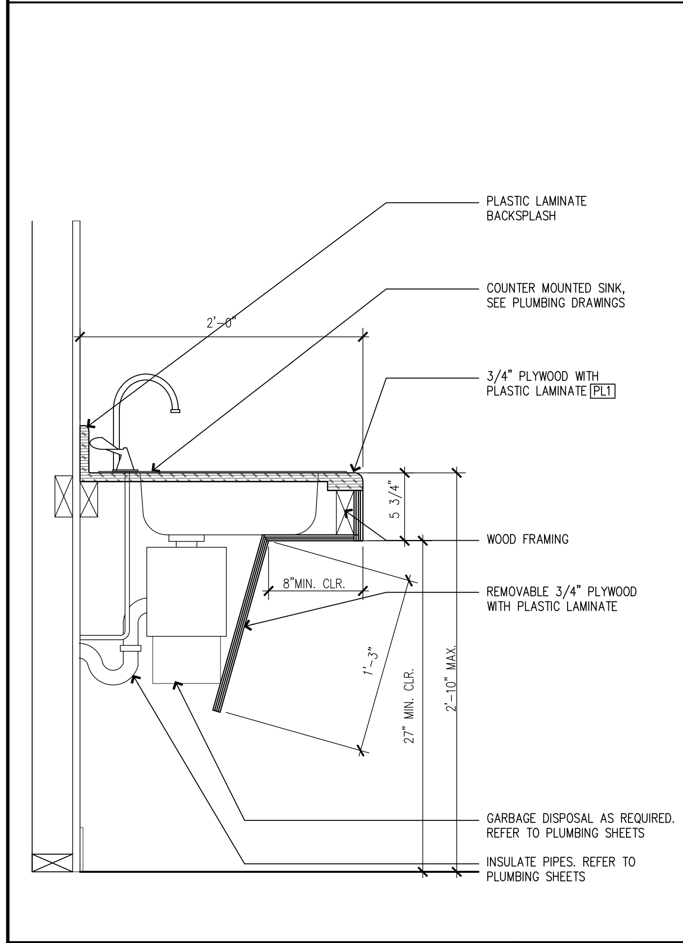
SECTION AT SINK
