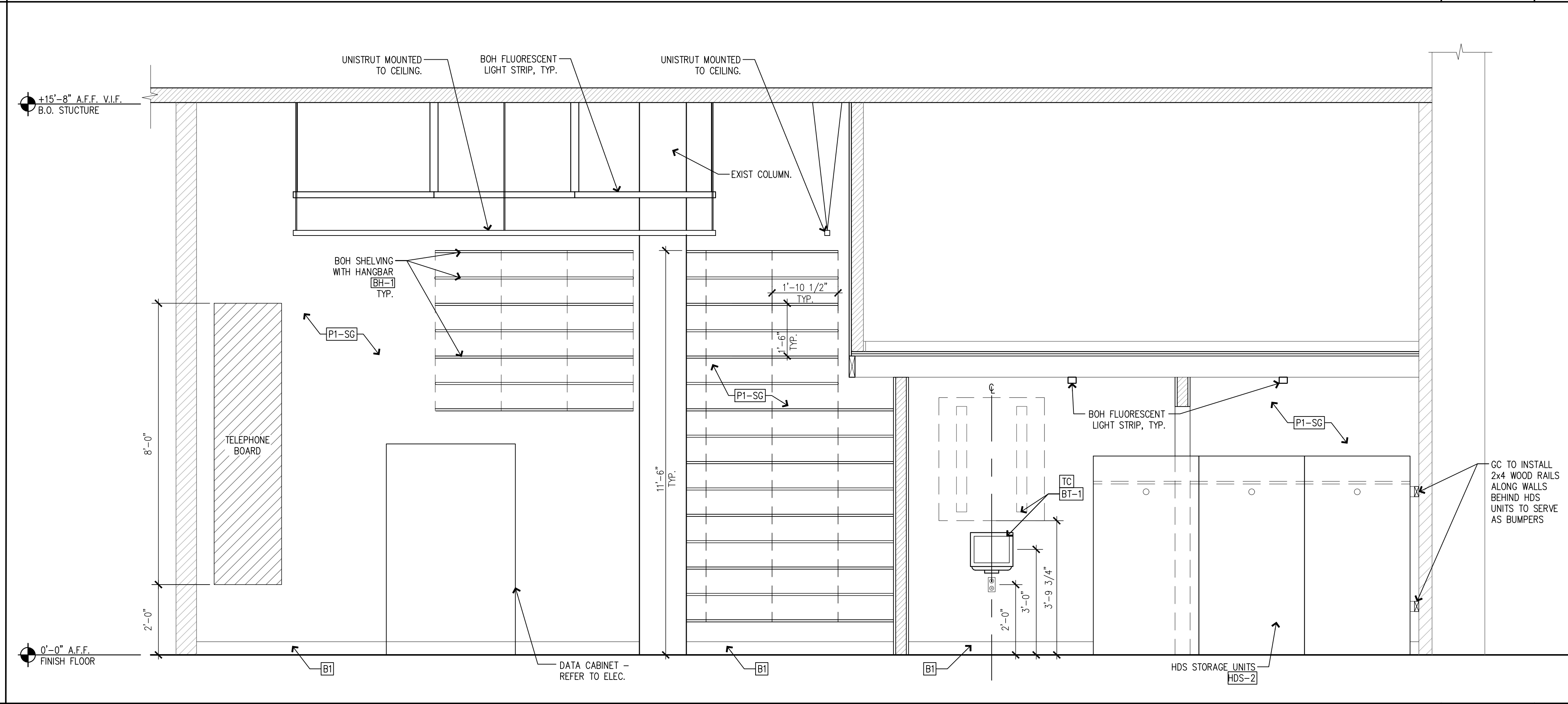
BOH AREA ELEVATION
