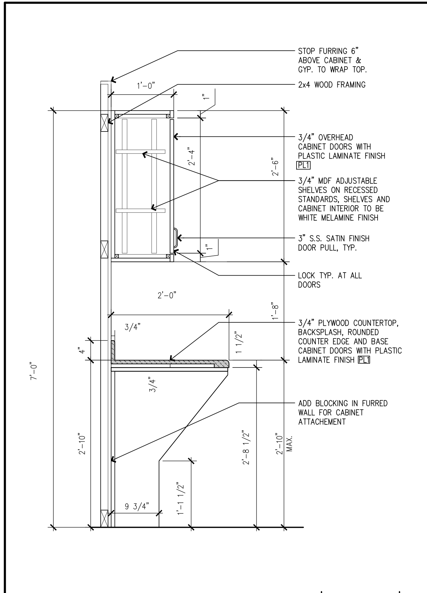
SECTION AT MANAGER'S DESK
