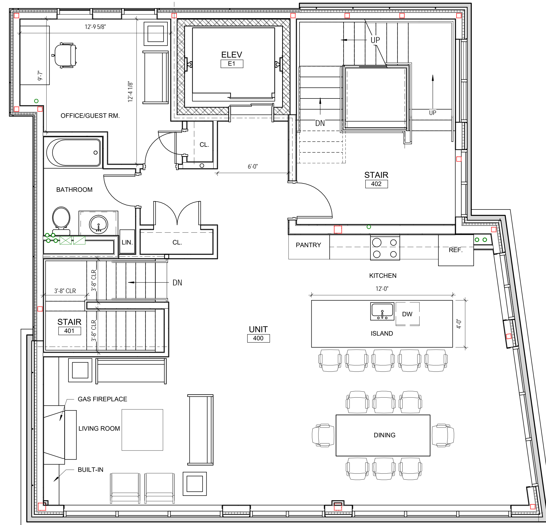
2 FOURTH FLOOR PLAN - Townhouse Marketing
