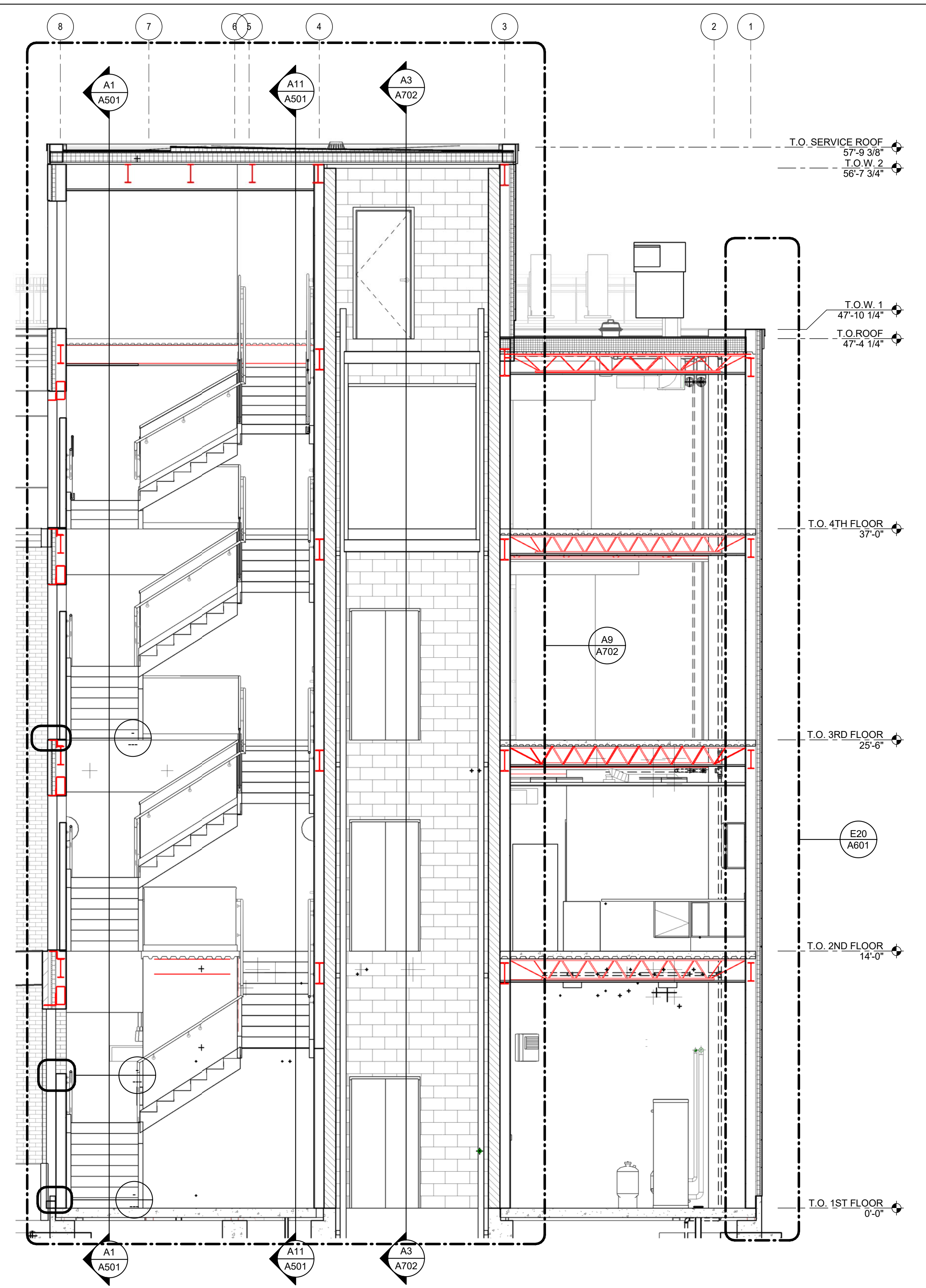
A11 BUILDING SECTION 1/4" = 1'-0"
