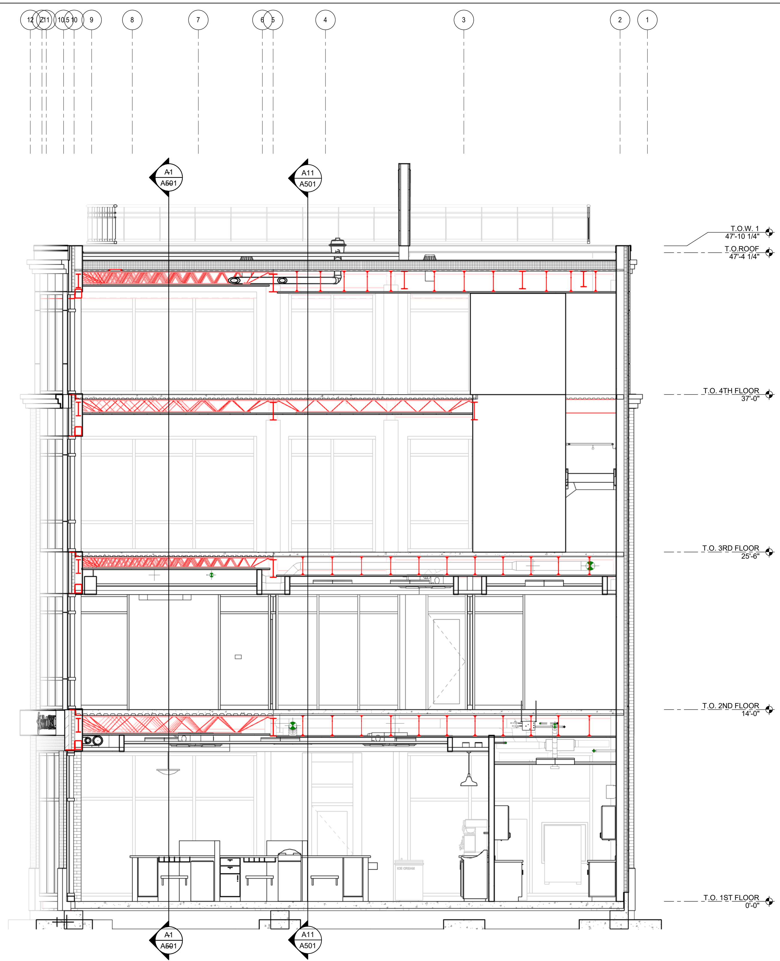
A1 BUILDING SECTION 1/4" = 1'-0"
