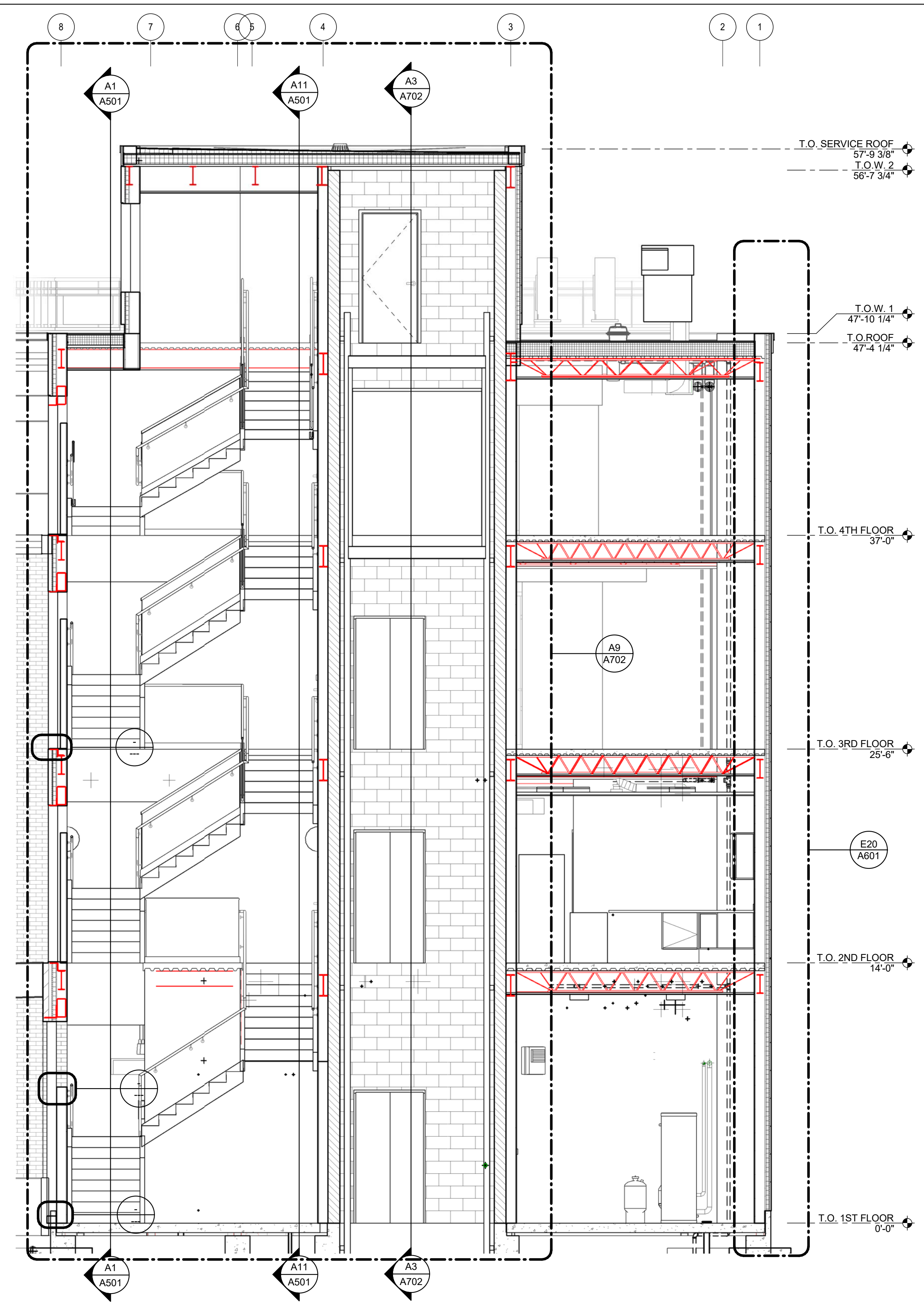
A11 BUILDING SECTION 1/4" = 1'-0"
