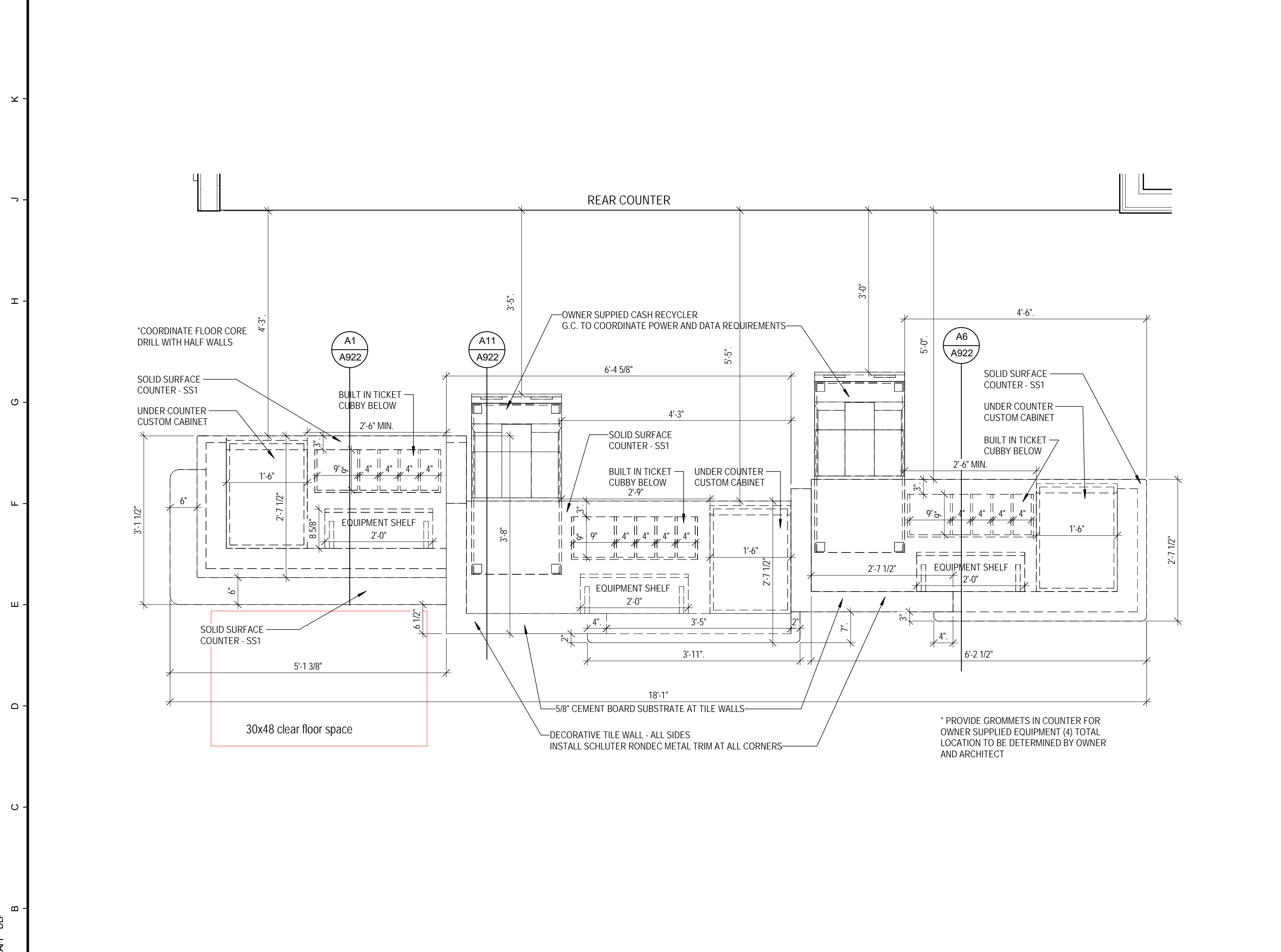
A1 ENLARGED PLAN AT TELLER POD 3/4" = 1'-0"
