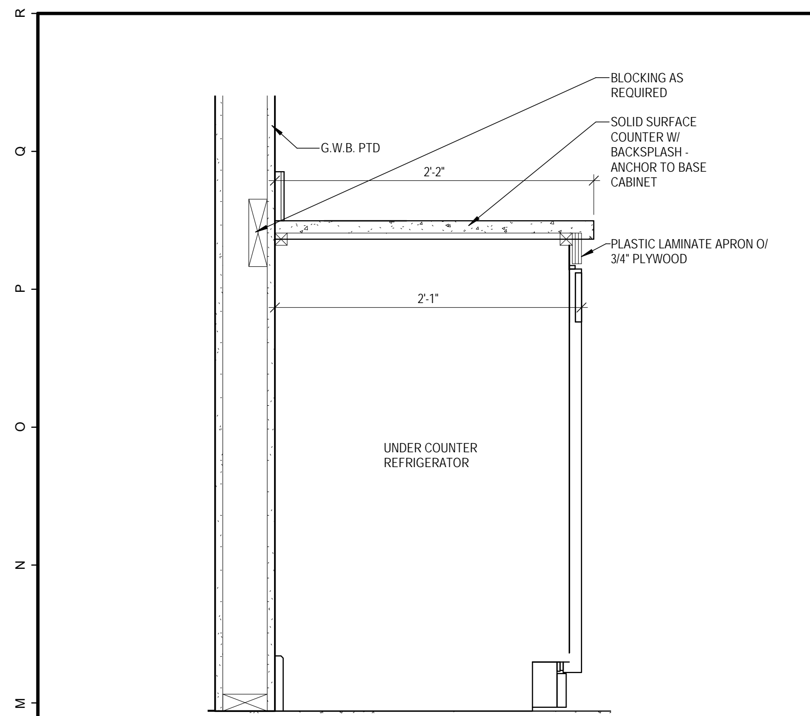
L1 UNDERCOUNTER REFRIGERATOR 1 1/2" = 1'-0"
