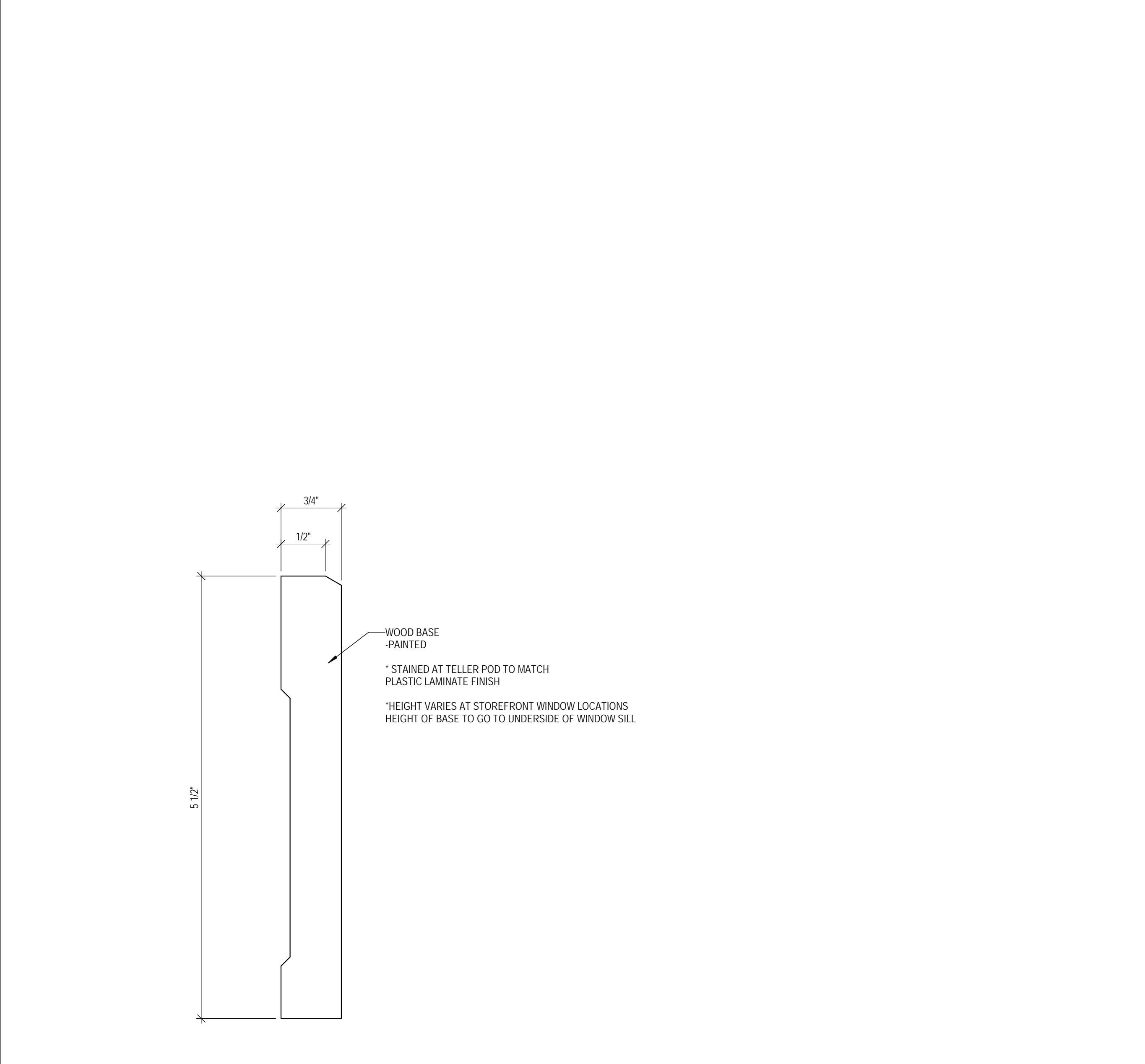
A12 WOOD BASE 1/2" = 1'-0"
