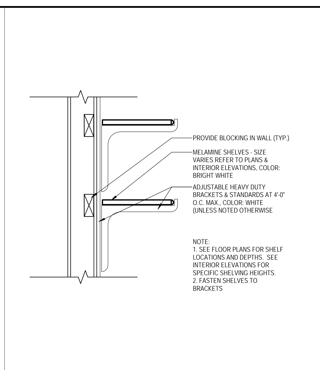
L17 ADJUSTABLE SHELVING DETAIL 1 1/2" = 1'-0"
