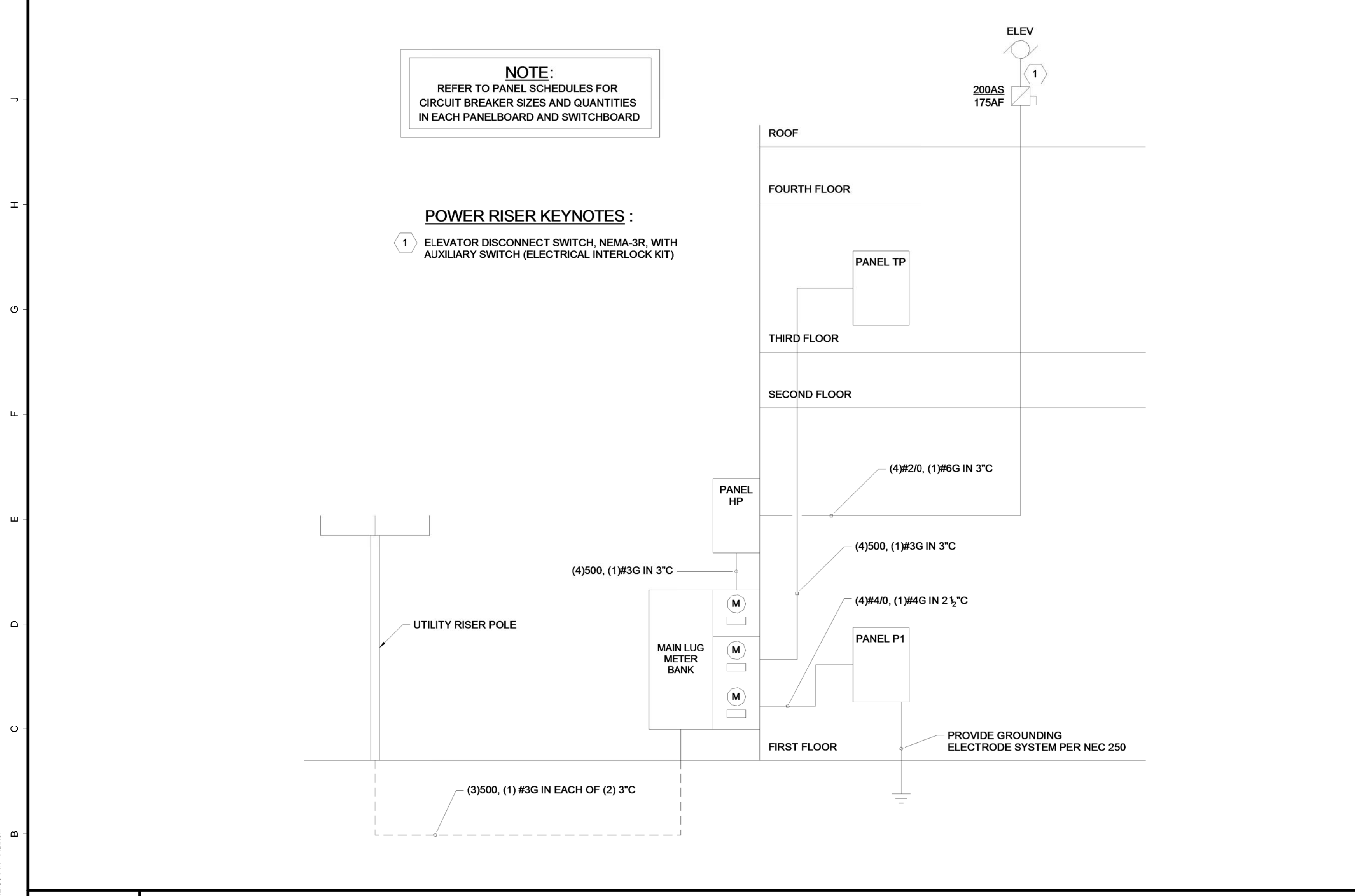
A1 POWER RISER DIAGRAM
