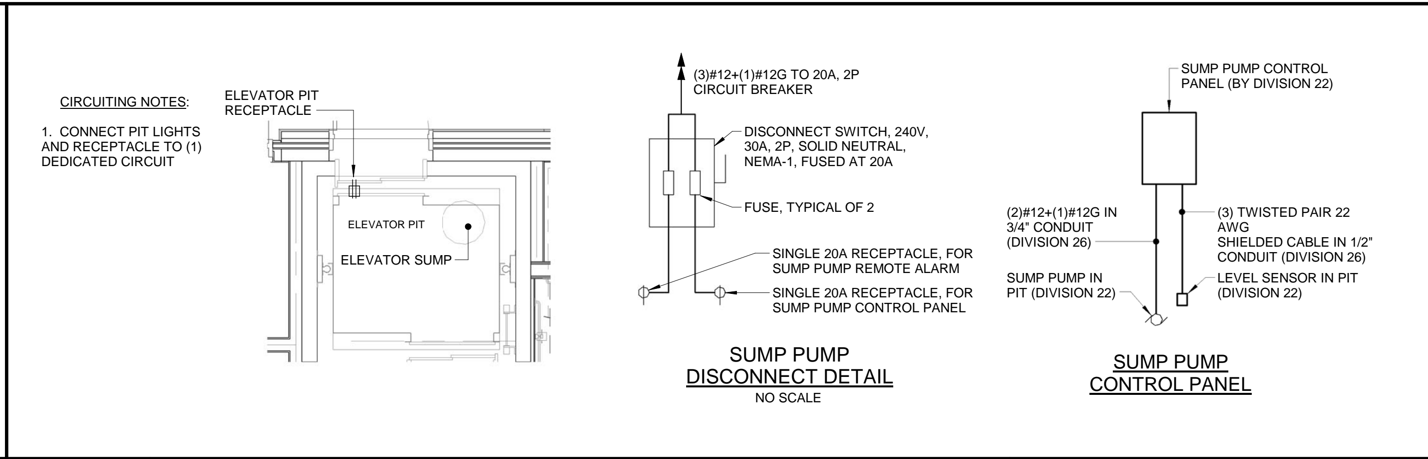
K6 ELEVATOR PIT DETAIL 1/4" = 1'-0"
