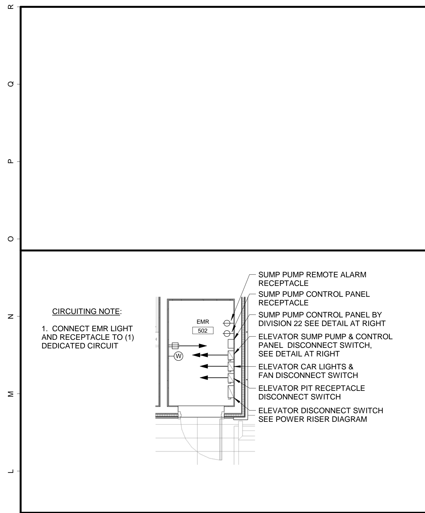
K1 ELEVATOR MACHINE ROOM DETAIL 1/4" = 1'-0"
