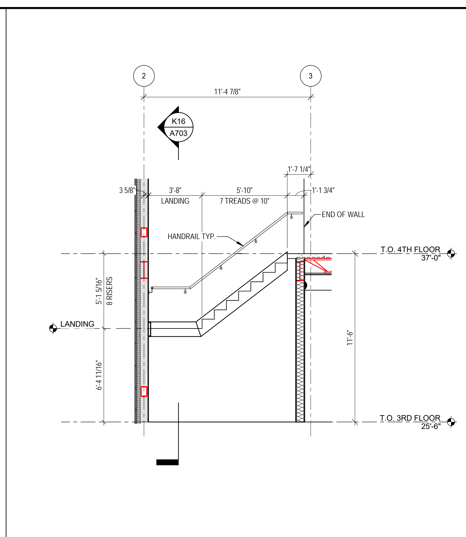
K11 STAIR SECTION - 5 1/4" = 1'-0"
