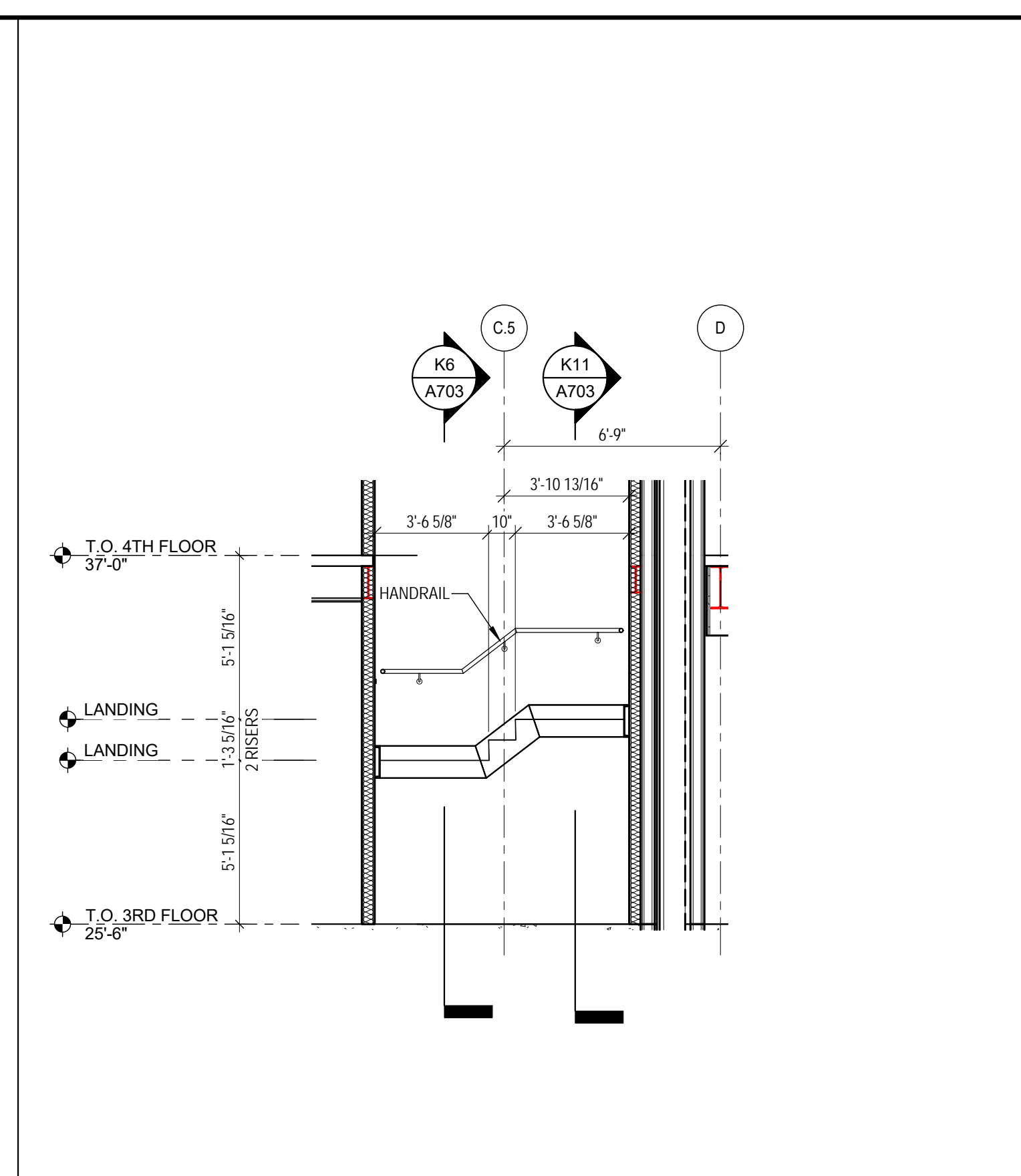
K16 STAIR SECTION - 6 1/4" = 1'-0"
