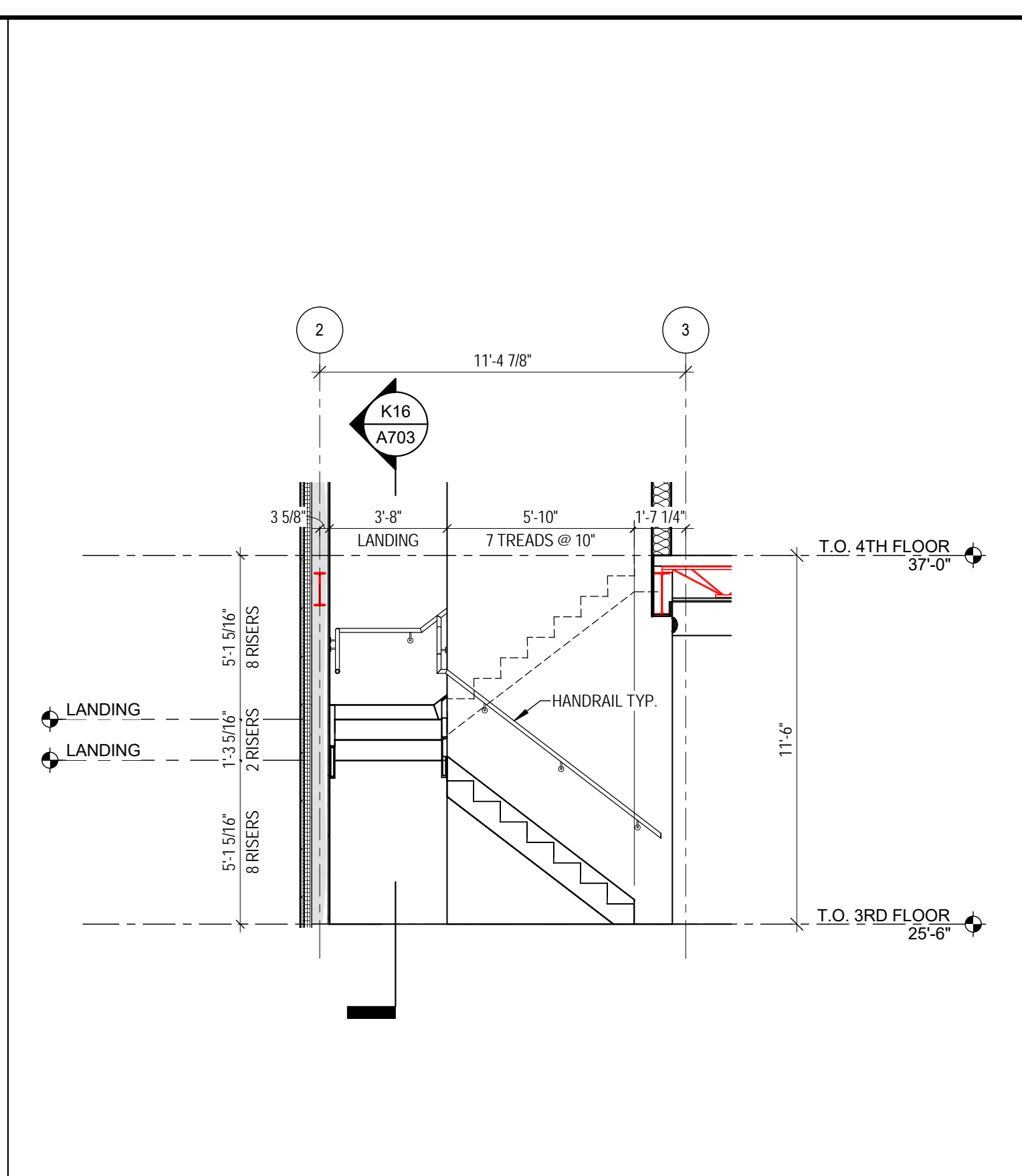
K6 STAIR SECTION - 4 1/4" = 1'-0"
