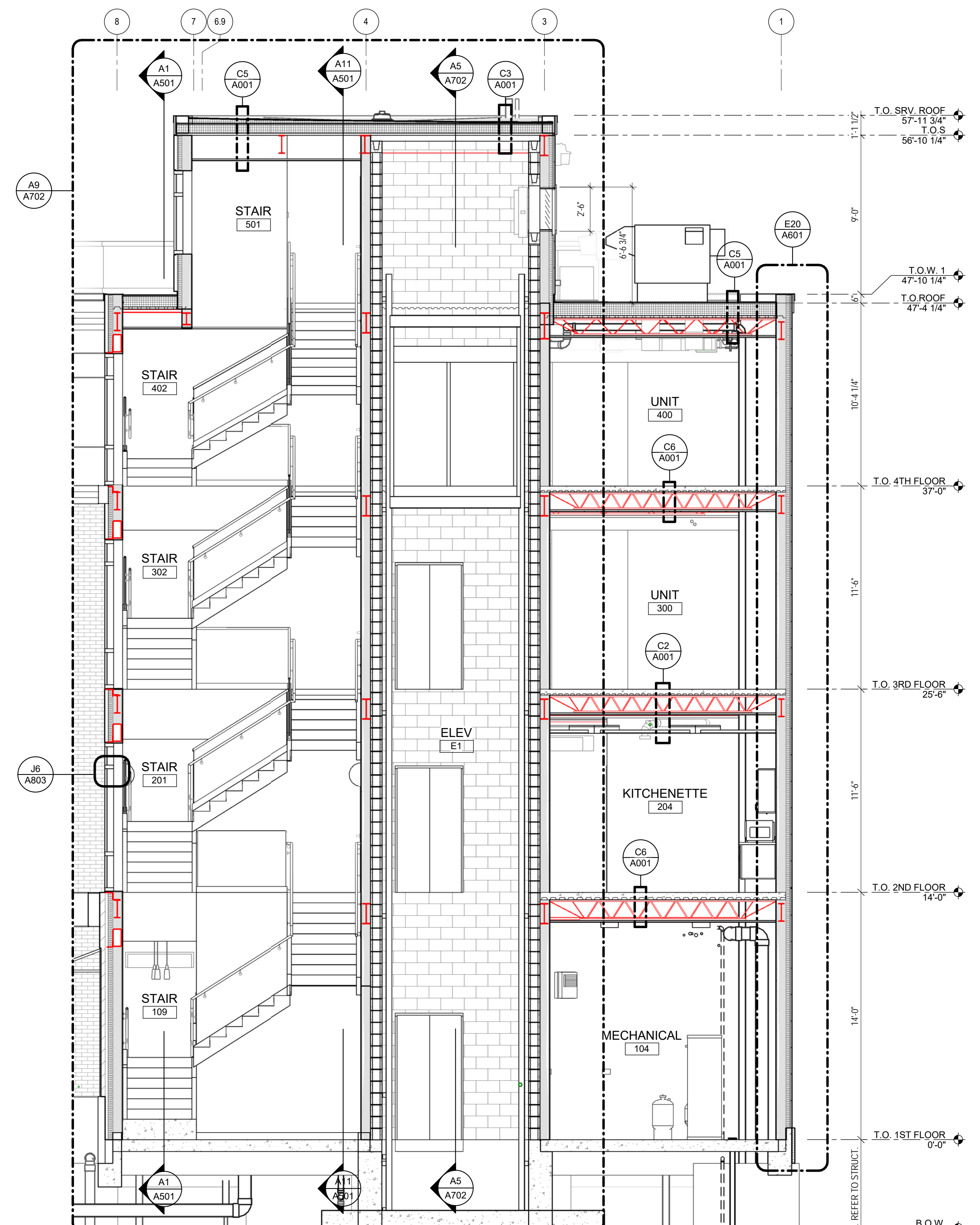
A11 BUILDING SECTION
