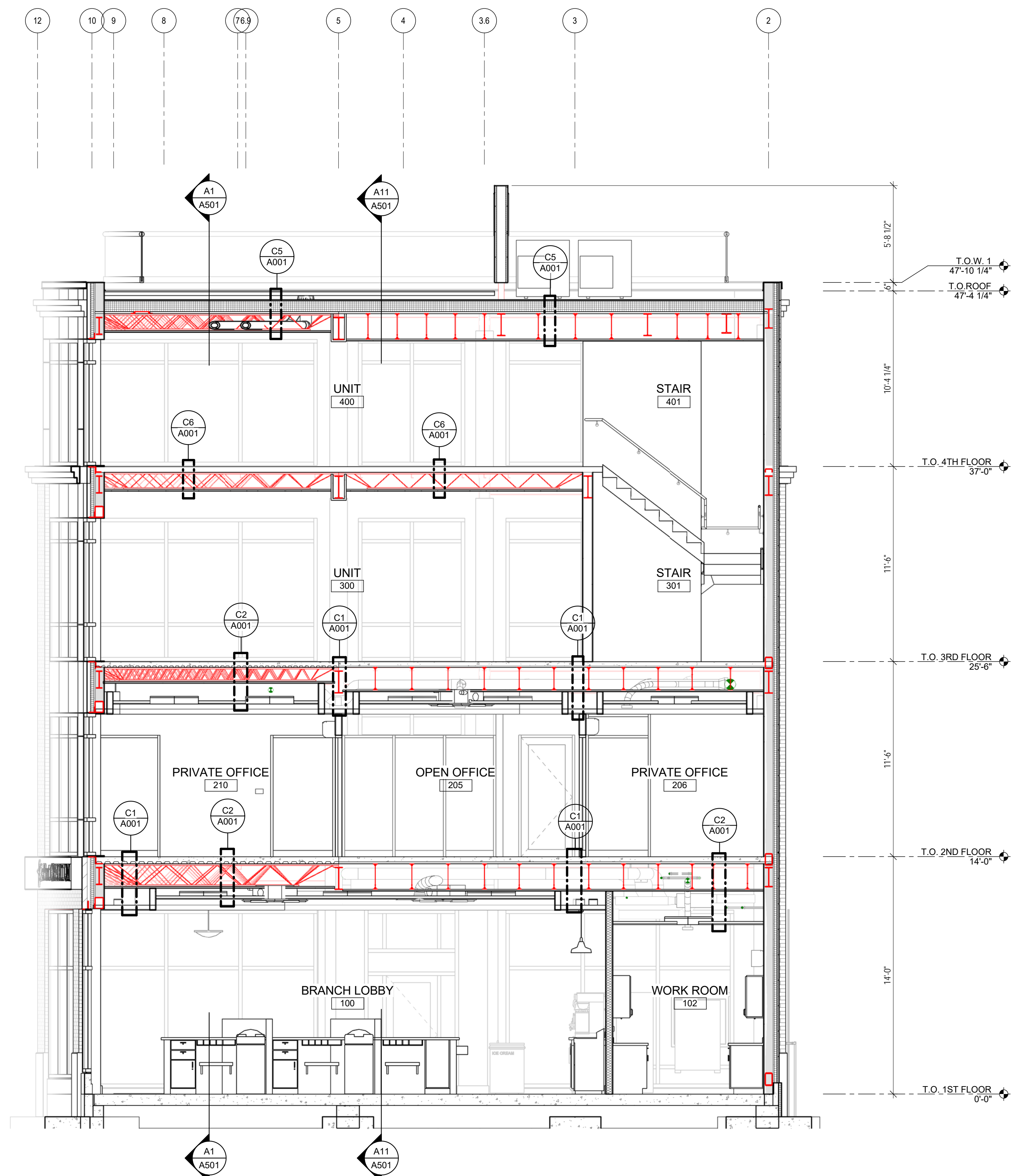
A1 BUILDING SECTION
