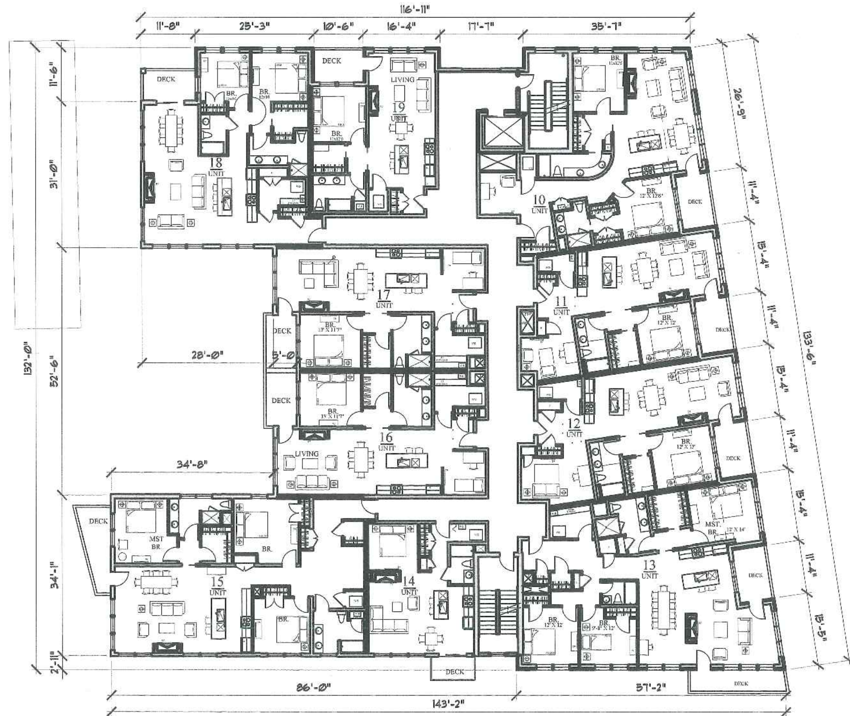
THIRD LEVEL PLAN SCALE: 1"=20'-0"
