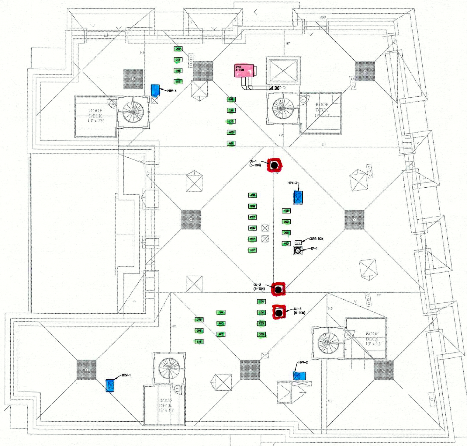
ROOF - DUCTWORK SCALE: 1/8"=1'-0"
